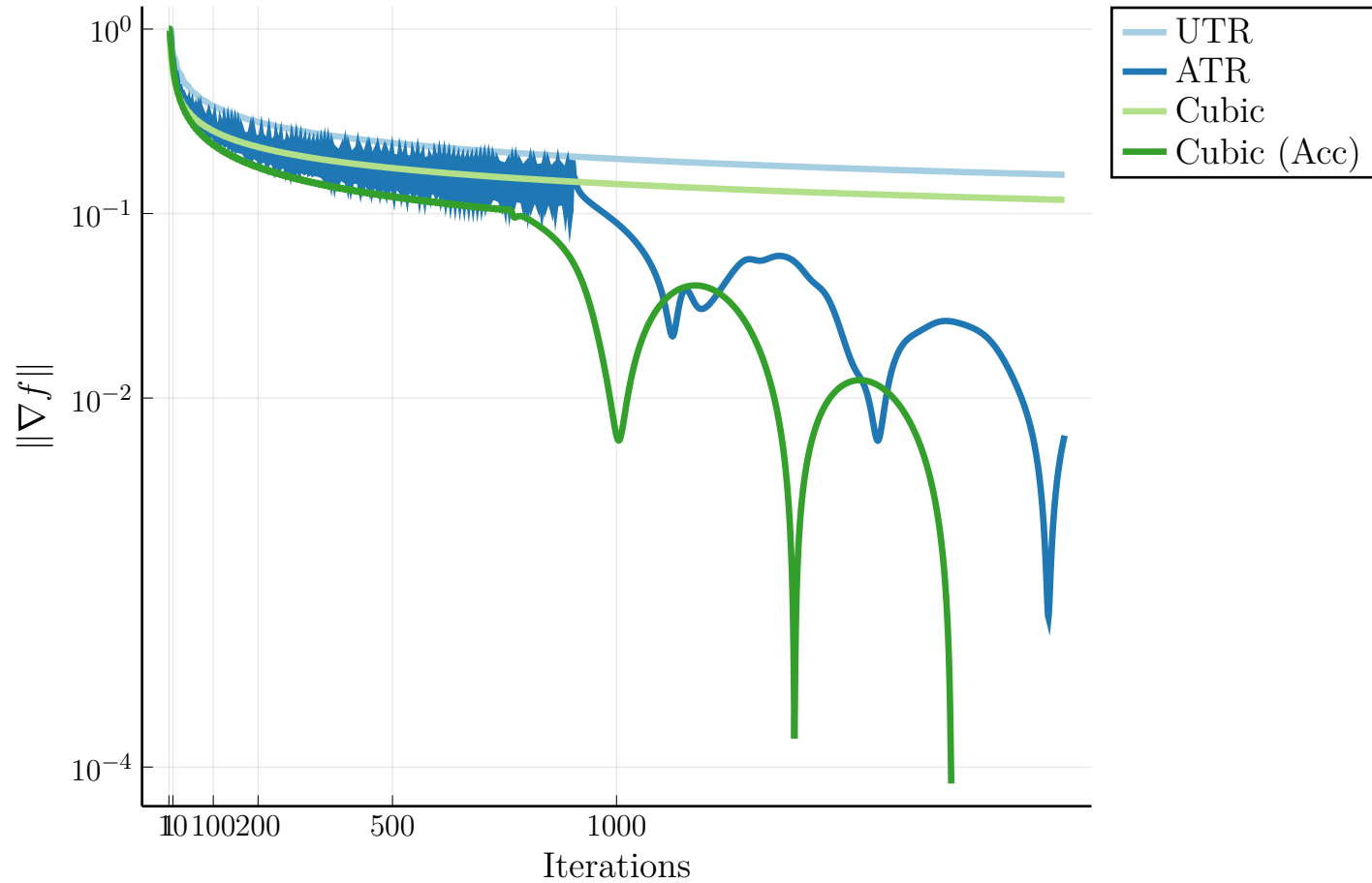
Nesterov's Lower Bound Function: n := 150, k := 100, p := 4
