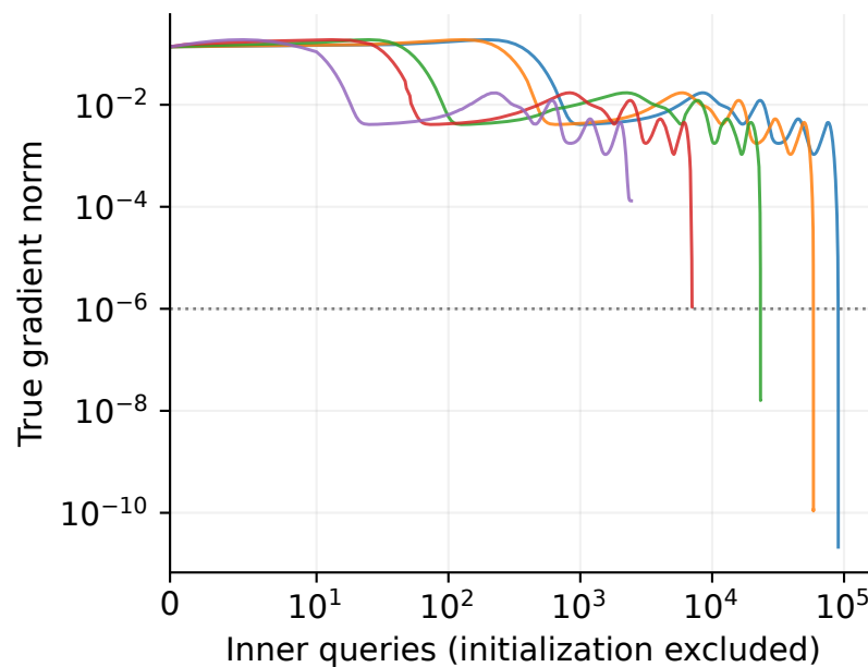
Effective L2 = 1
