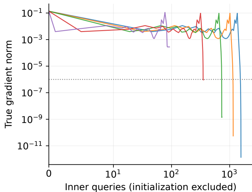
Effective L2 = 0.0001
