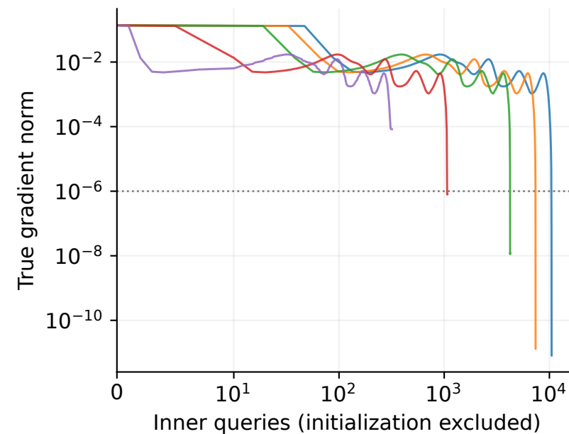
Effective L2 = 0.01
