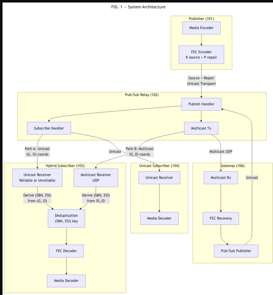
FIG. 1 – System Architecture
