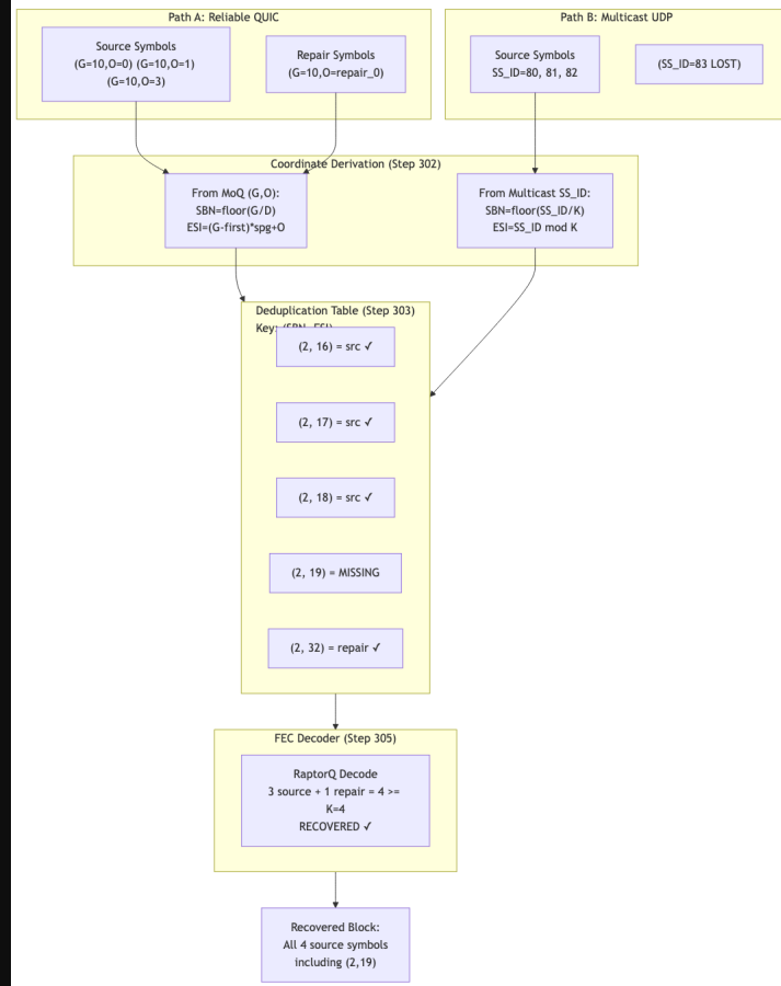
FIG. 3 — Multi-Path FEC Symbol Combining
