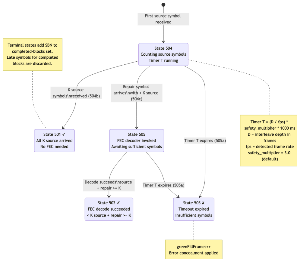
FIG. 5 — FEC Block Lifecycle State Machine
