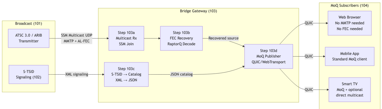
FIG. 1 — Broadcast-to-Unicast Bridge Architecture
