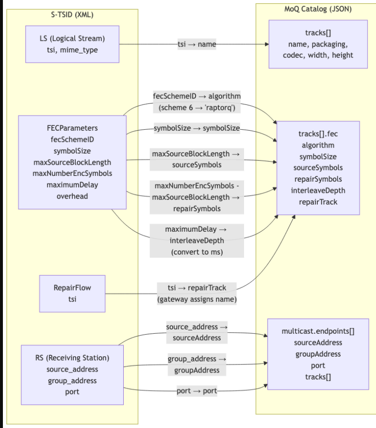
FIG. 3 – S-TSID to MoQ Catalog Field Mapping
