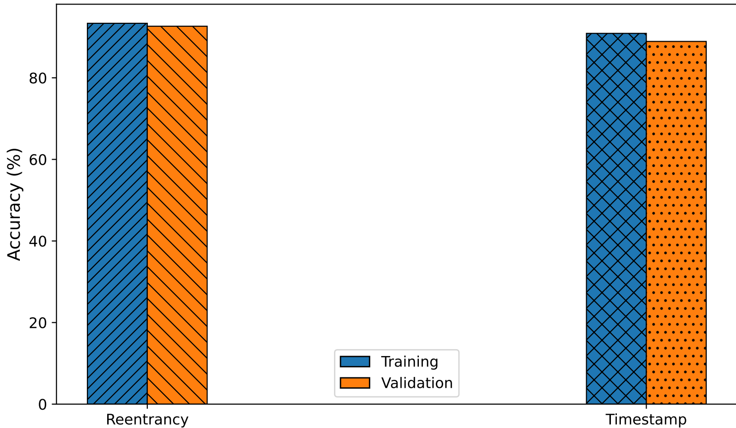
Final Training vs Validation Accuracy
