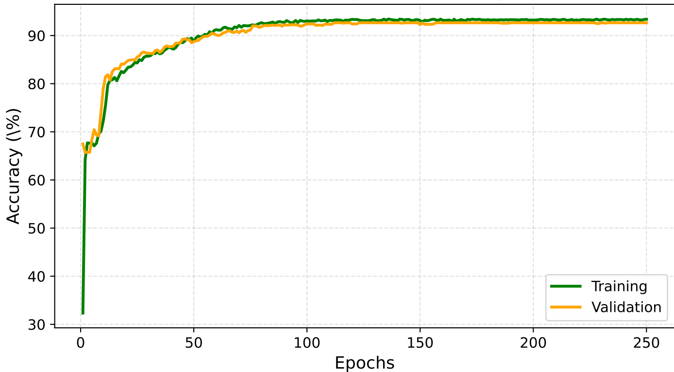
Accuracy over Epochs (Reentrancy)
