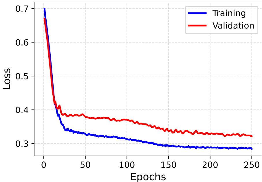
Loss over Epochs (Timestamp)
