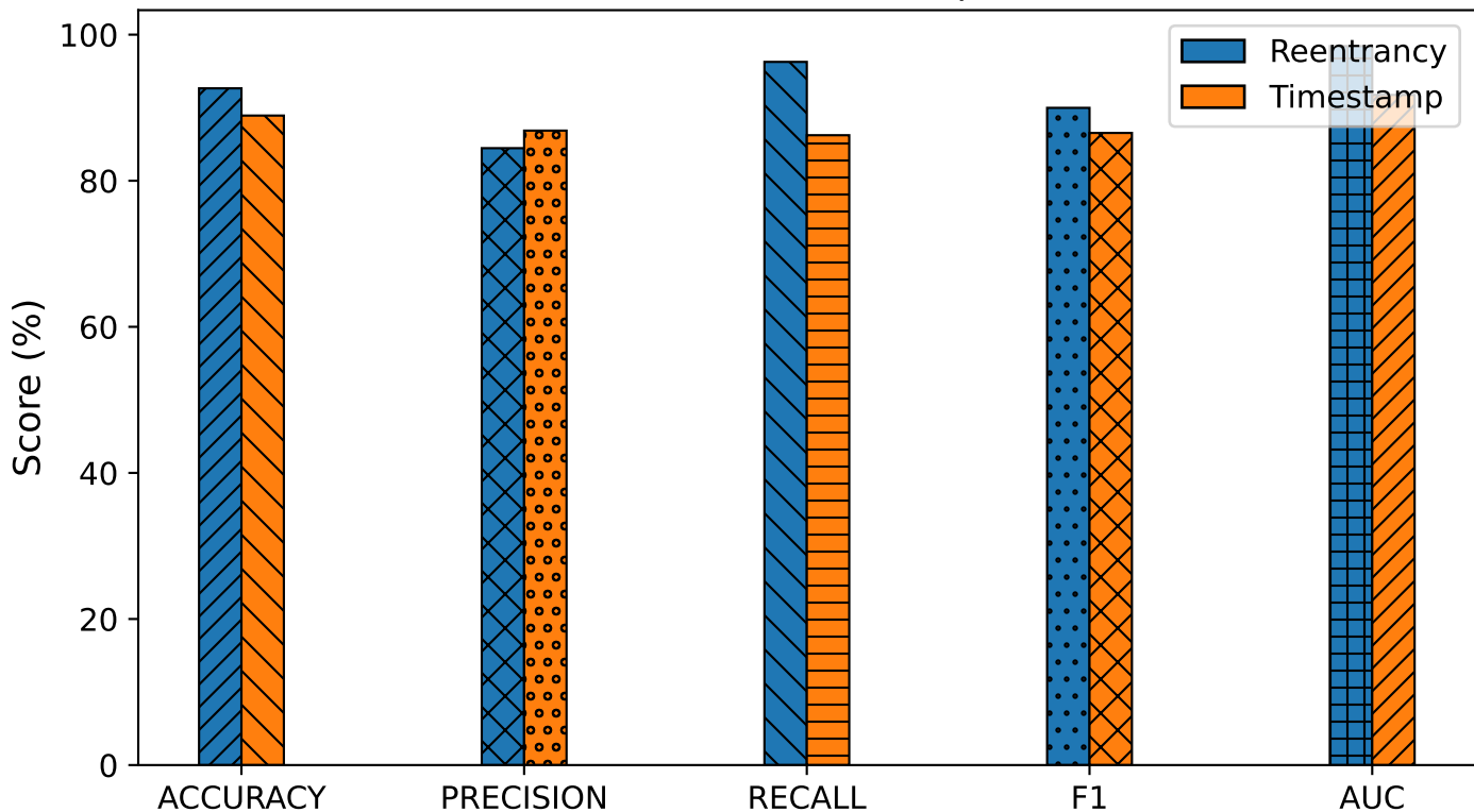
Evaluation Metrics Comparison
