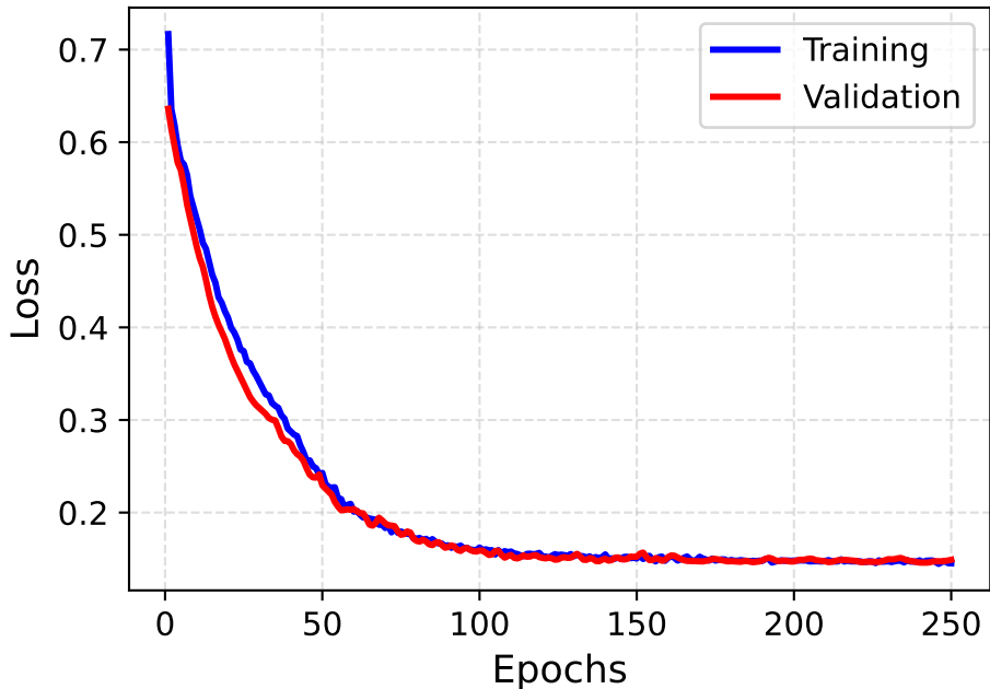
Loss over Epochs (Reentrancy)
