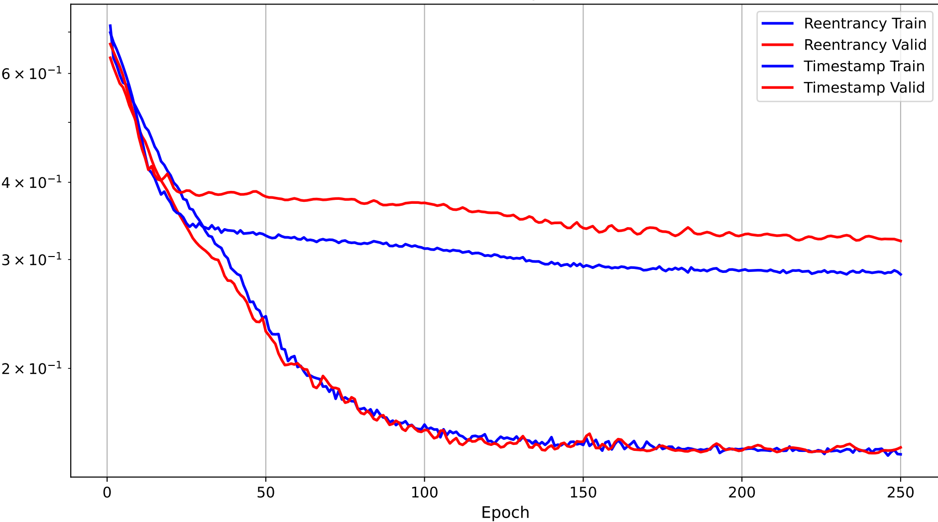
Loss over Epochs
