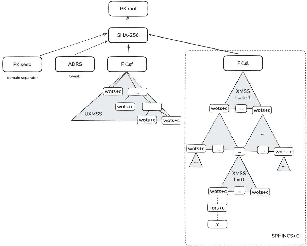
Figure 1: SHRINCS architecture
