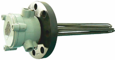
Oil Sump Heater with Flame Proof Enclosure
