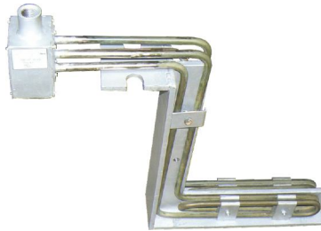
Heater for Lead Melting for Battery Manufacturing
