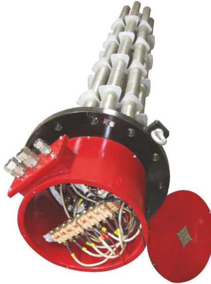
Oil Outflow Heater of Indirect Type, Range 2KW to 120KW
