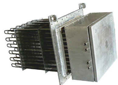
Purge Air Heater
