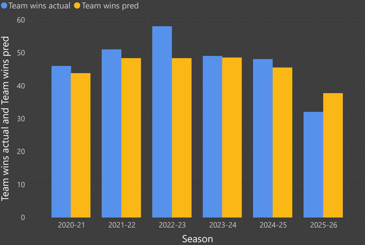
Team wins actual and Team wins pred by Season
