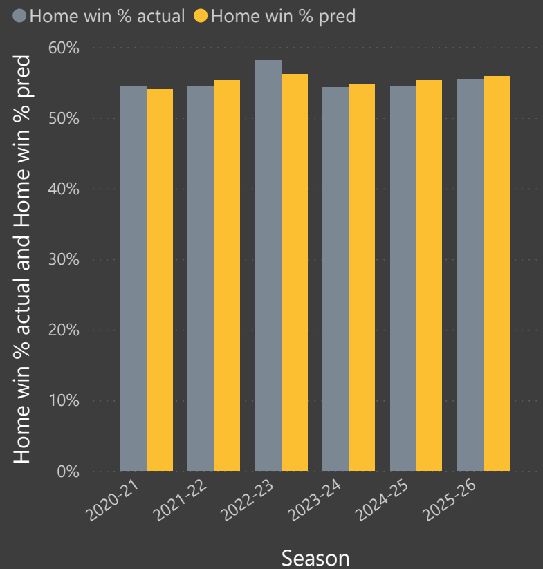
Home win % actual and Home win % pred by season
