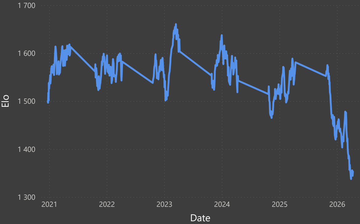
Elo by Date
