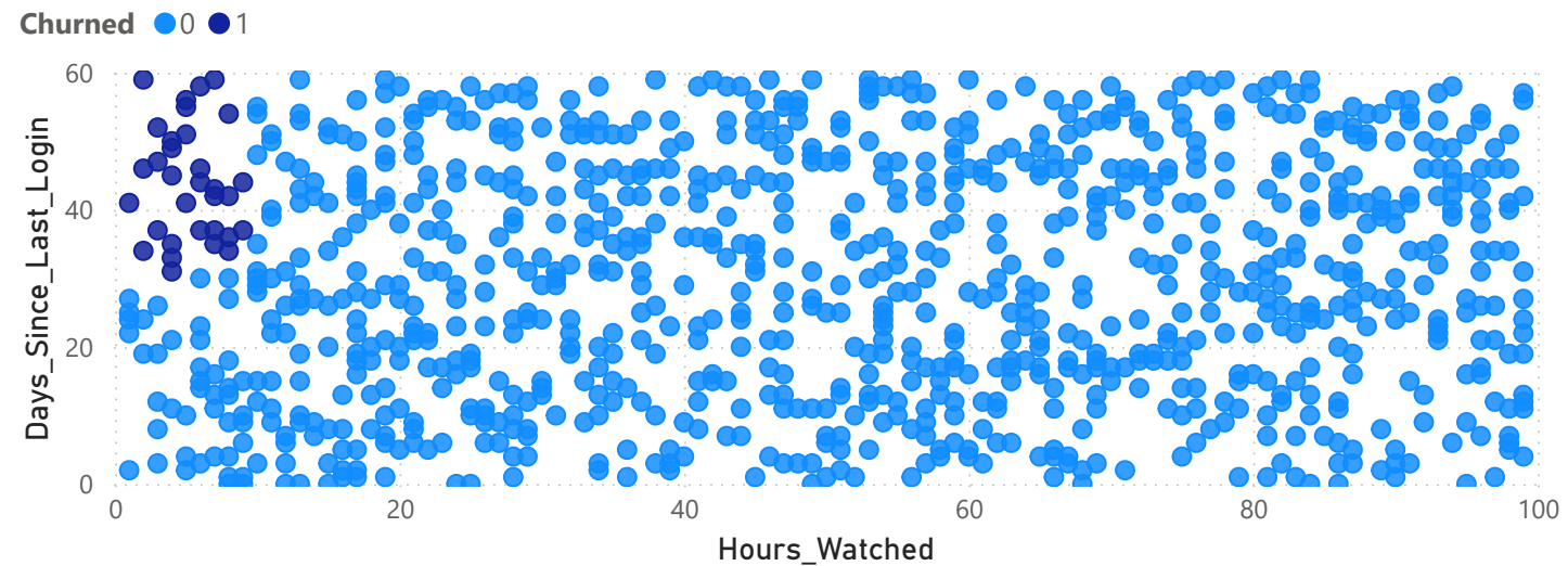
Churned, Hours_Watched and Days_Since_Last_Login
