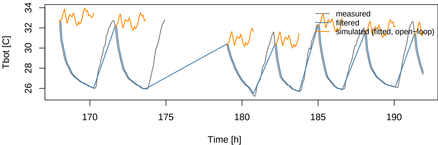
Fitted vs. measured Tbot
