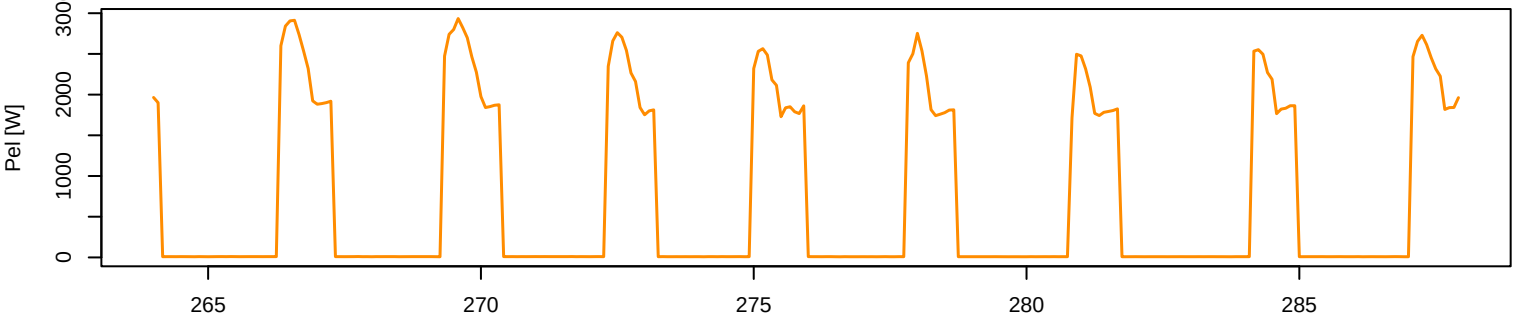
GSHP on/off switch
