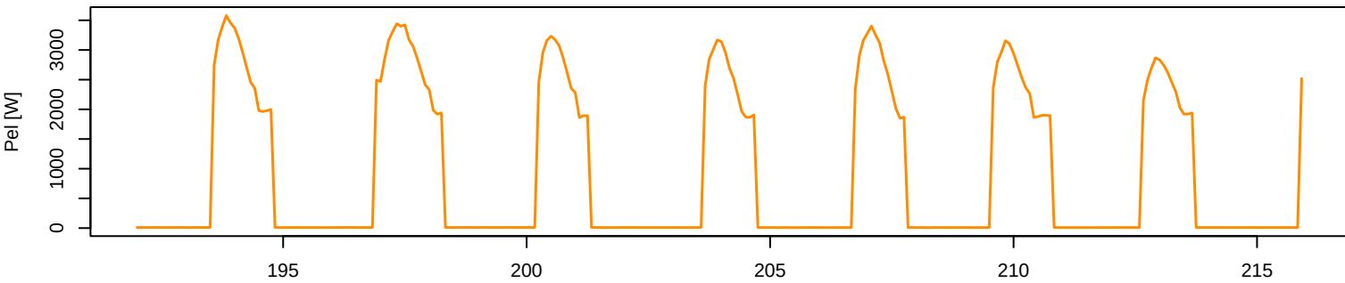
GSHP on/off switch
