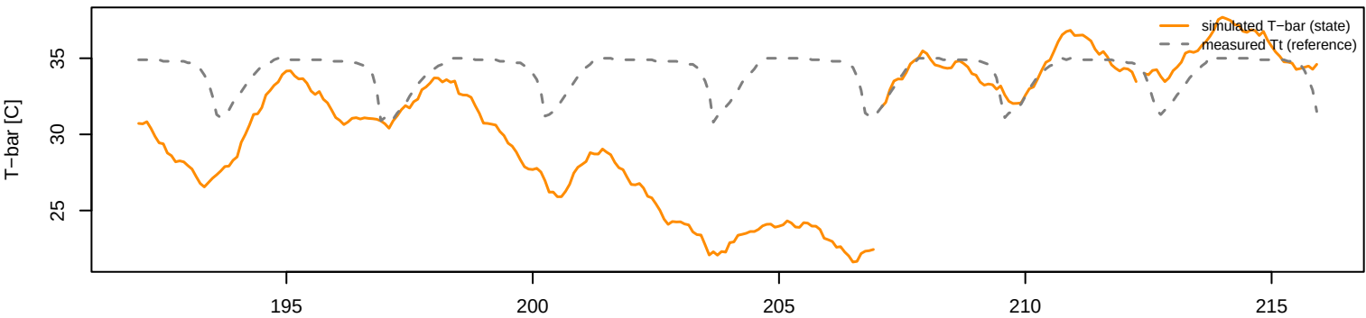
Simulated vs. measured Tb
