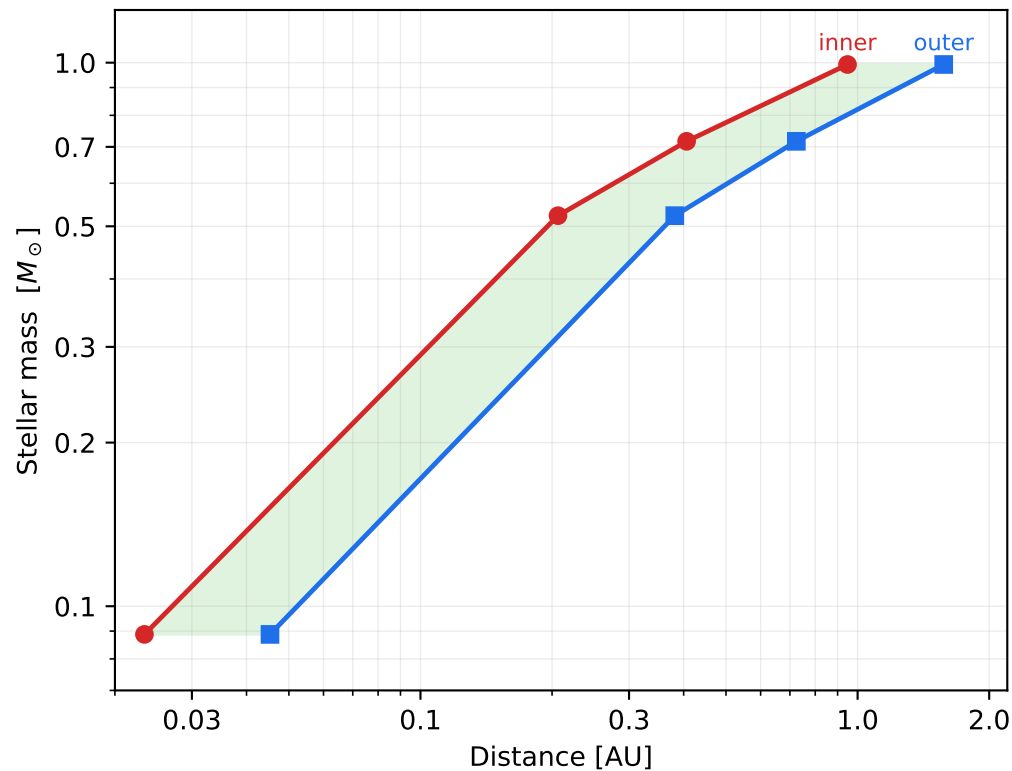
(b) HZ distances (Baraffe et al. 1998, 5 Gyr)
