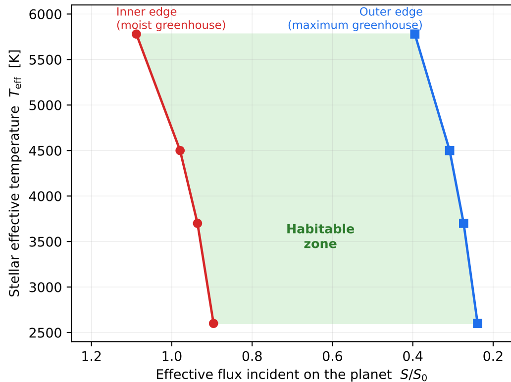
(a) HZ fluxes
