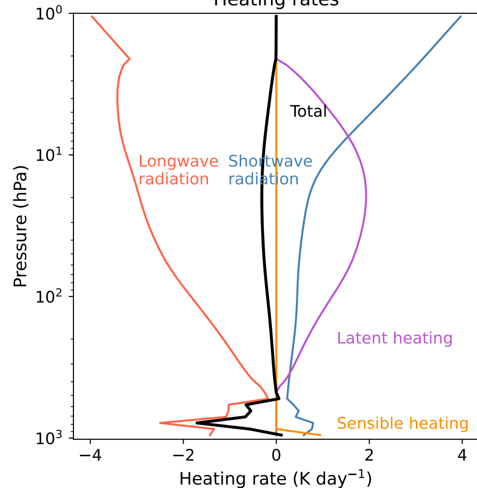
Heating rates
