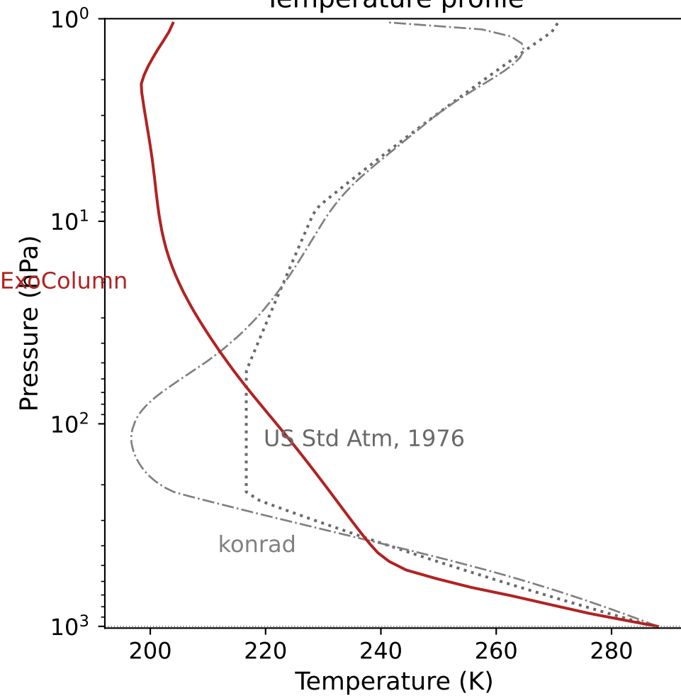
Temperature profile
