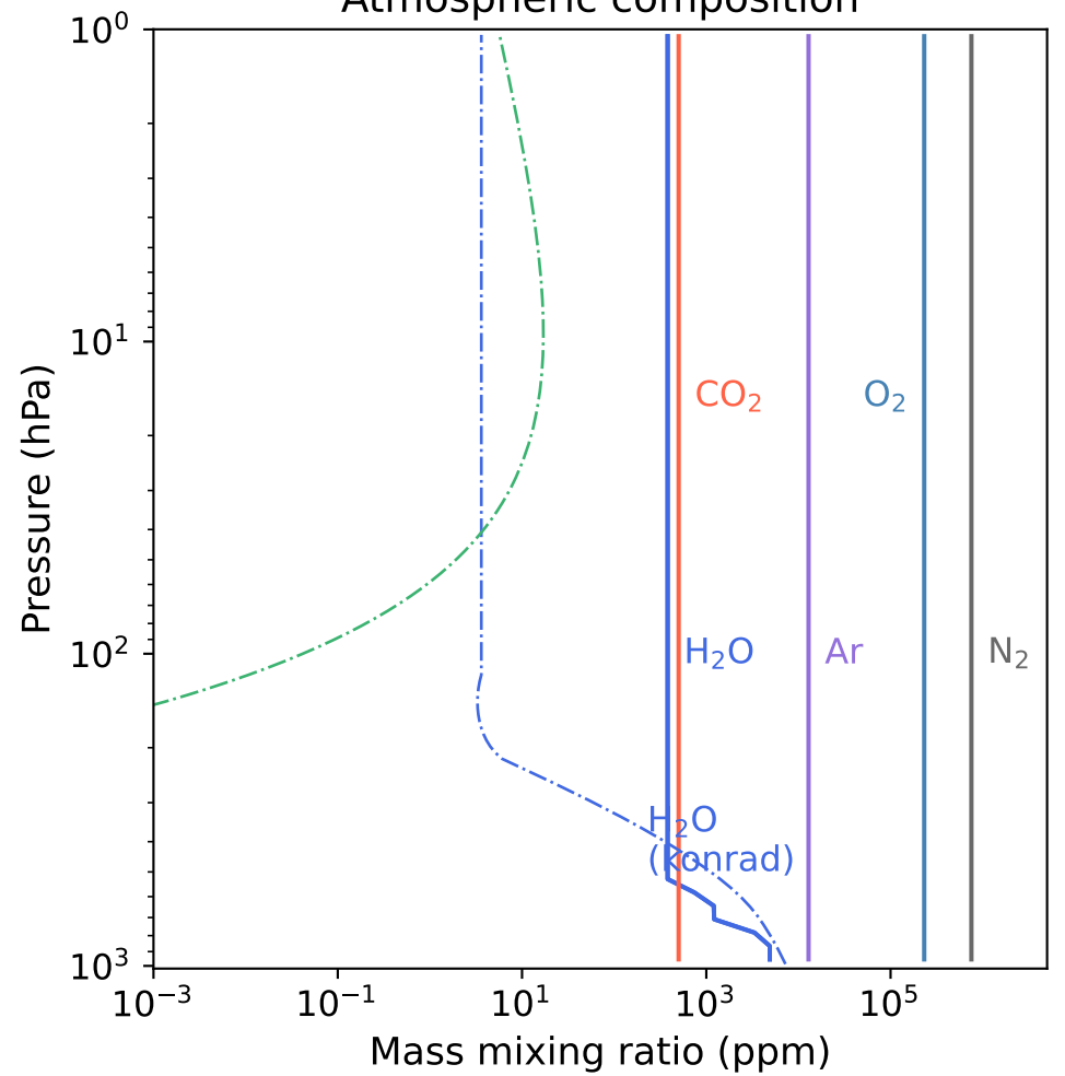
Atmospheric composition
