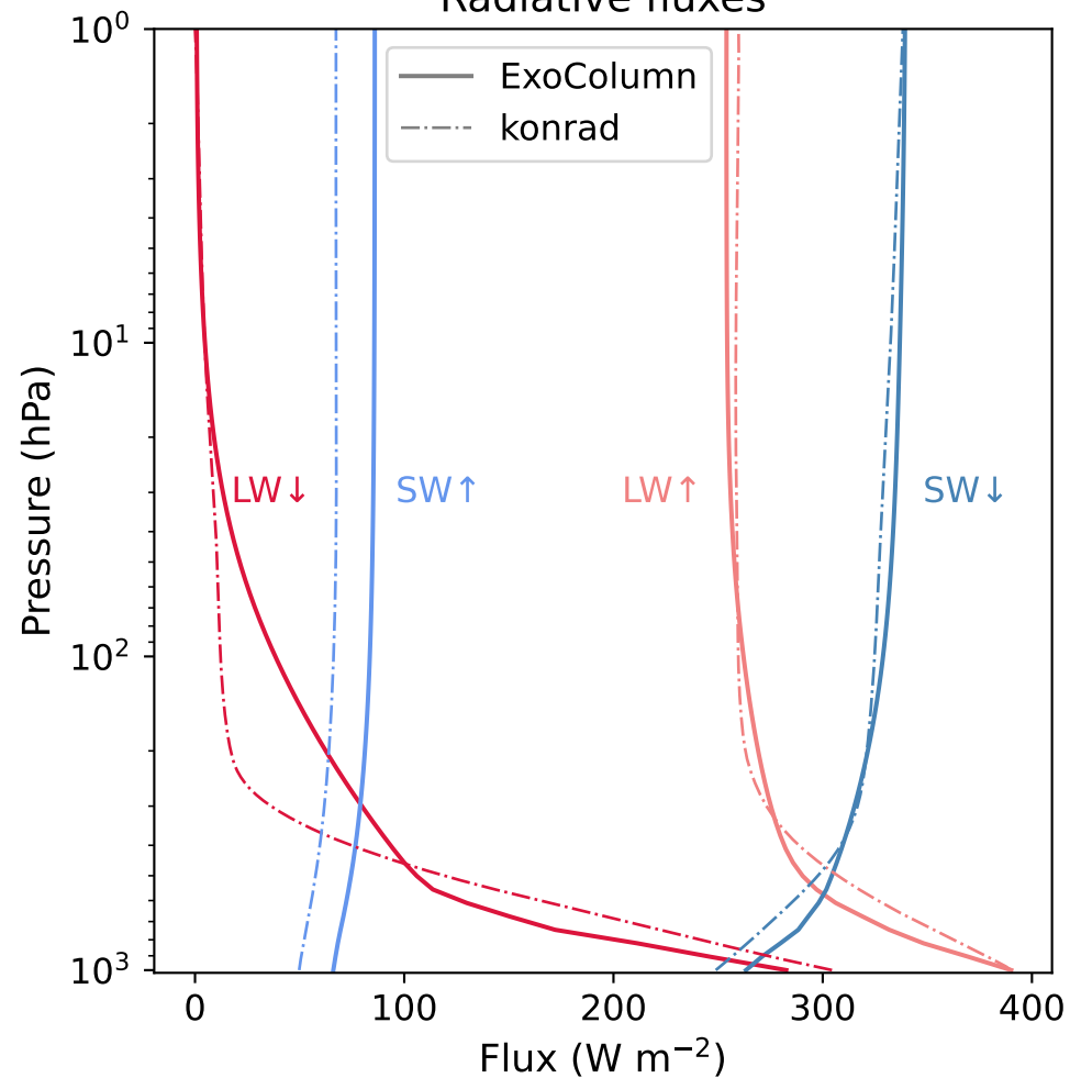
Radiative fluxes
