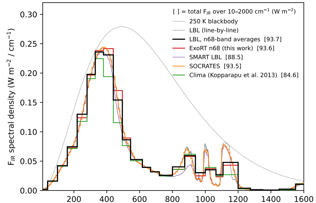
Outer HZ: early Mars T_s = 250 K (dry, 2 bar 95% \text{CO}_2 / 5% \text{N}_2 , Mars gravity)
