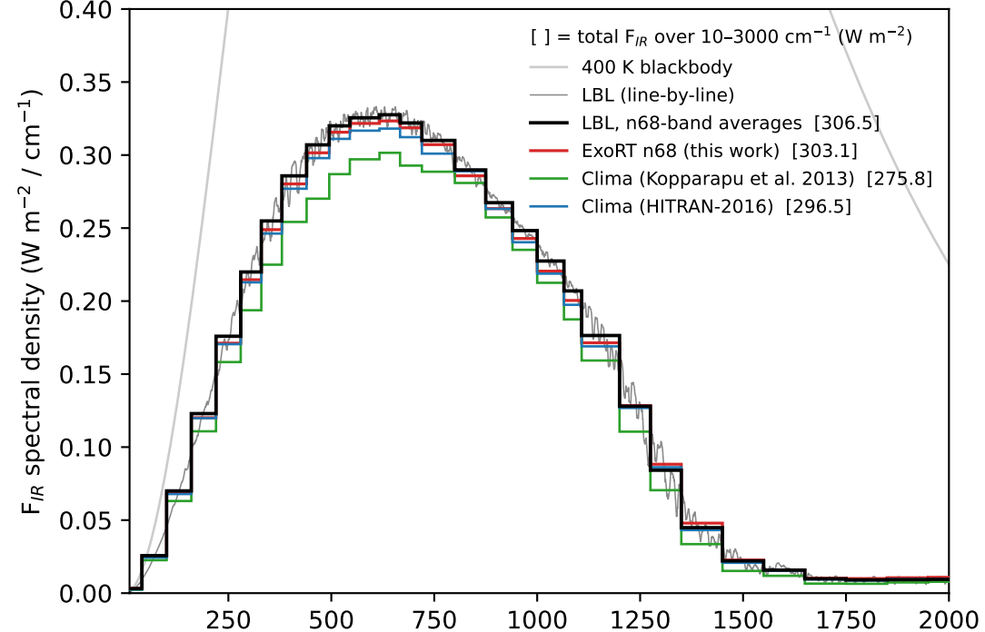
Inner HZ: dense H_2O T_s = 400 K (4 bar N_2 + H_2O , p_s = 6.46 bar)
