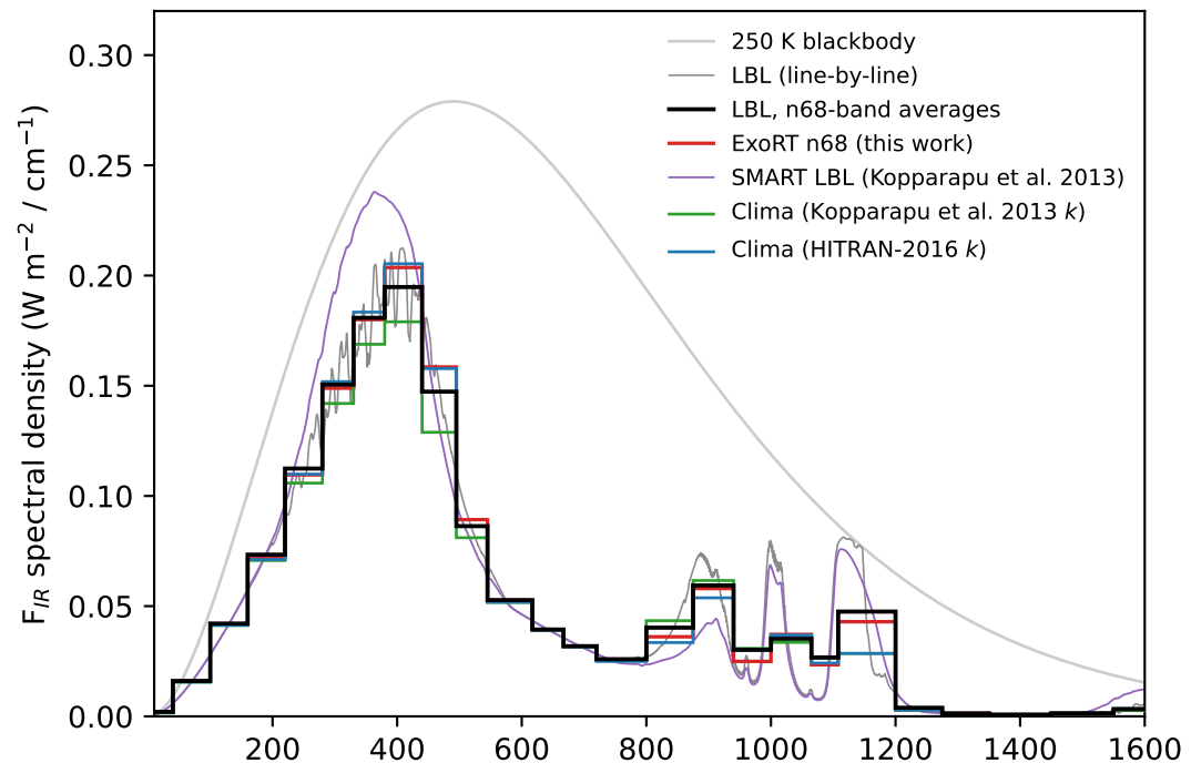
Outer HZ: early Mars T_s = 250 K (2 bar 95% \text{CO}_2 / 5% \text{N}_2 , Mars gravity)
