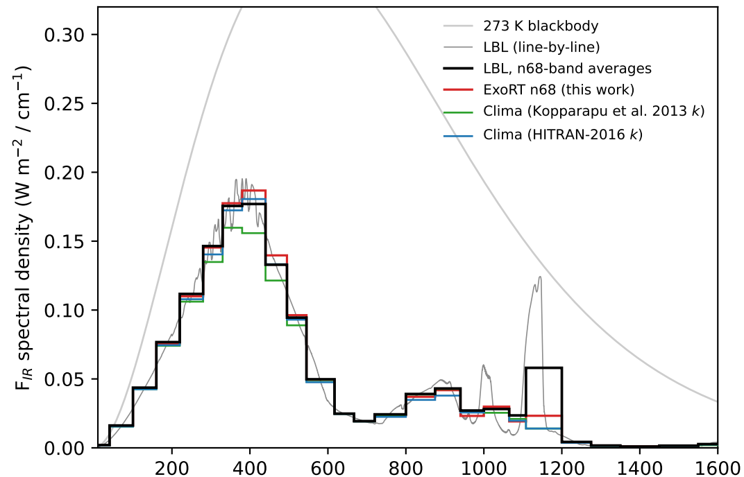
Outer HZ: max-greenhouse T_s = 273 K ( p\text{CO}_2 = 8.87 bar + 1 bar \text{N}_2 )
