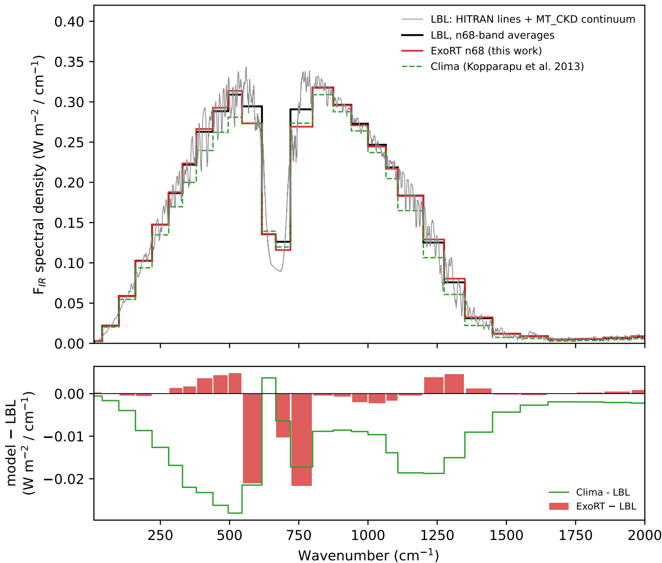
Clear-sky OLR, saturated T_s = 300 K column (1 bar N_2 + 330 ppm CO_2 + H_2O )
