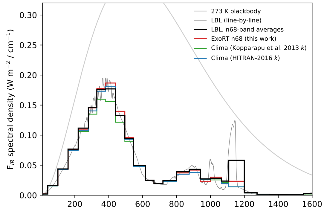
Outer HZ: max-greenhouse T_s = 273 K ( pCO_2 = 8.87 bar + 1 bar N_2 )
