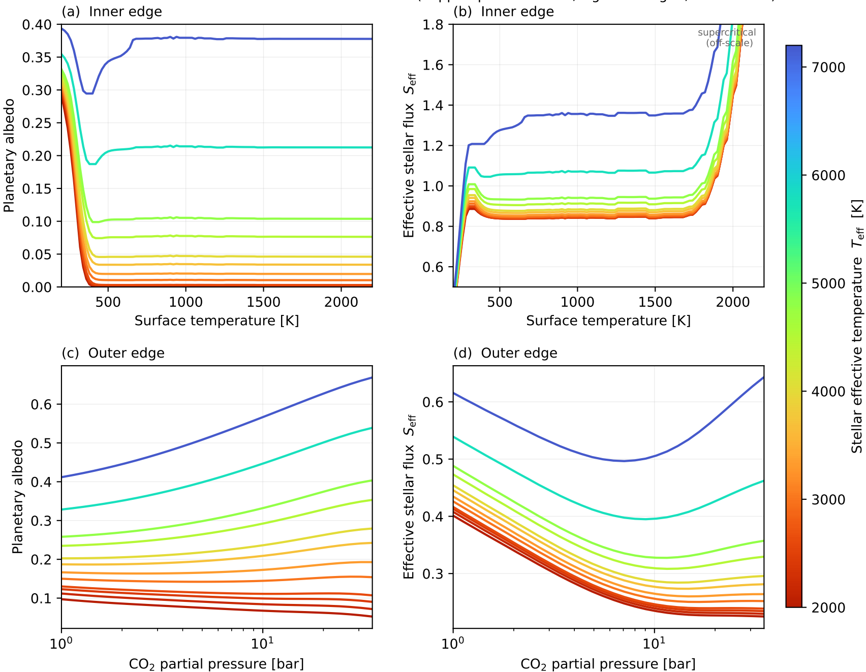
ExoColumn habitable-zone limits vs host star (Kopparapu et al. 2013, Fig. 6 analogue; F-G-K-M set)
