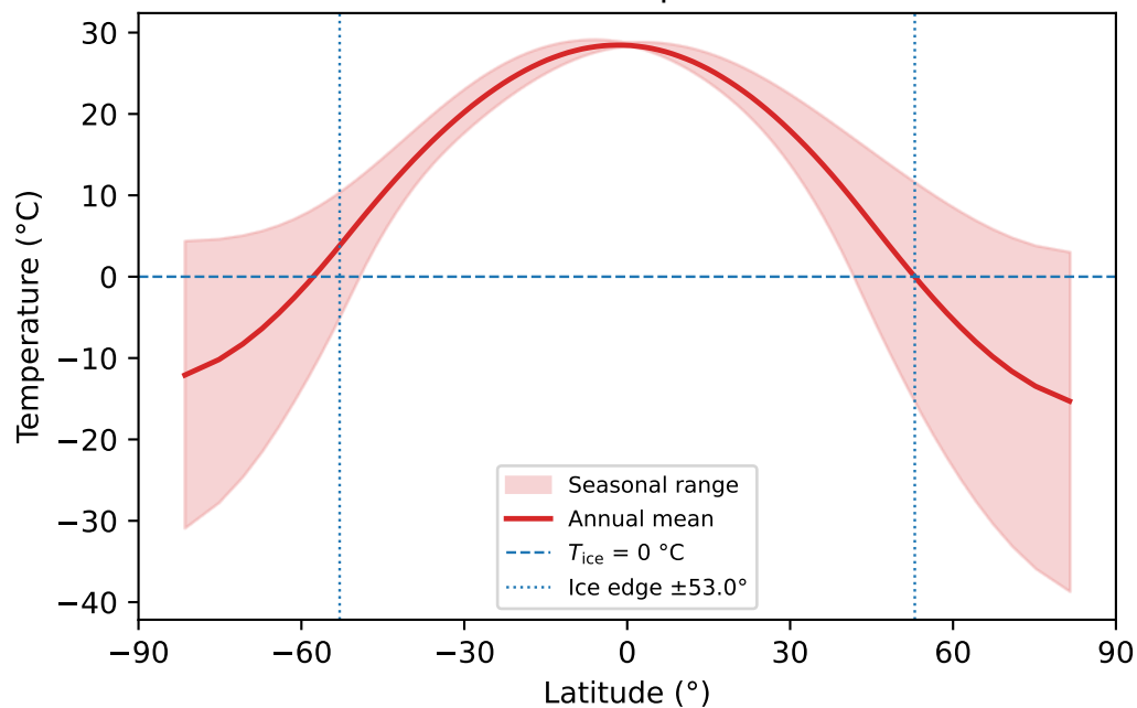
Annual-mean energy balance
