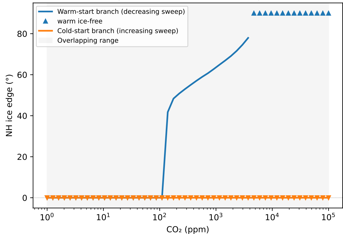
NH ice edge (triangle = ice-free / snowball endpoint)
