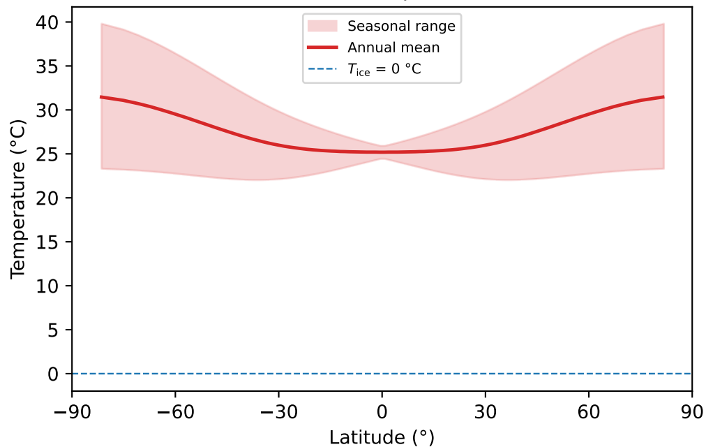
Annual-mean energy balance
