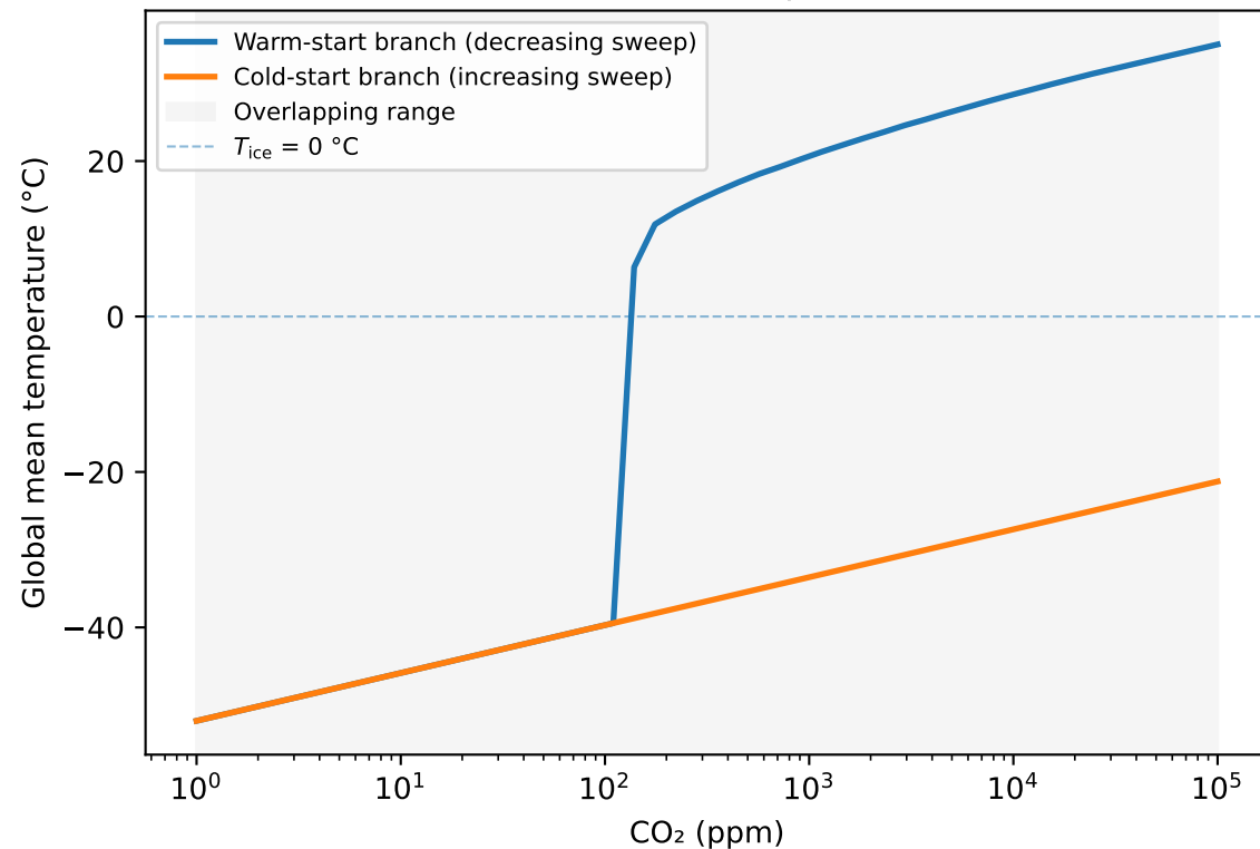
Global mean temperature
