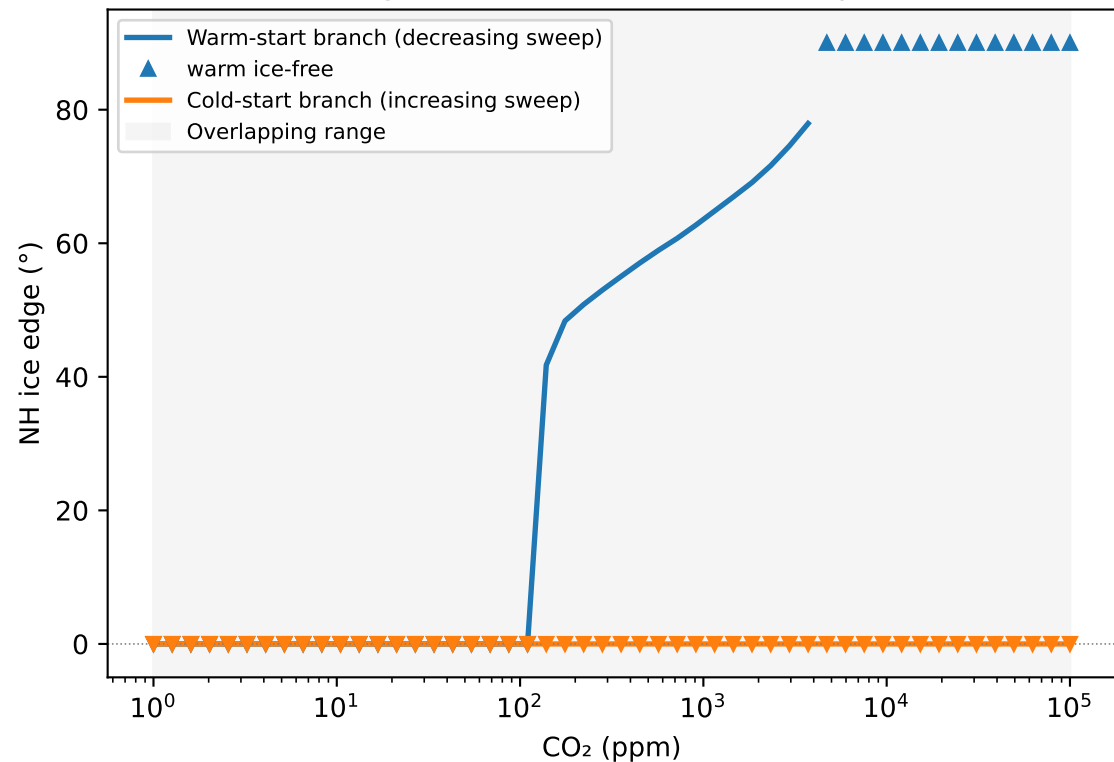
NH ice edge (triangle = ice-free / snowball endpoint)
