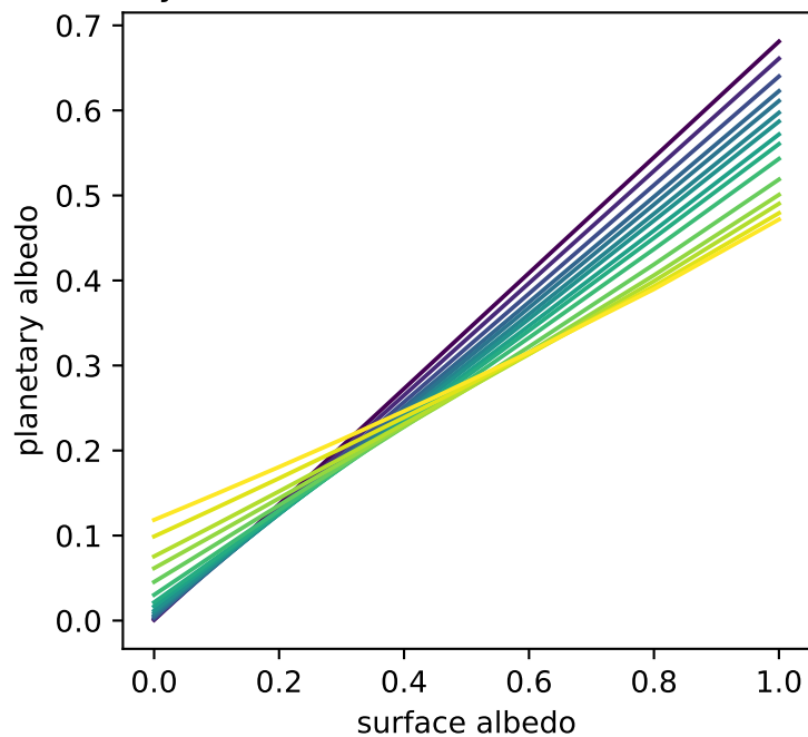
Planetary albedo vs surface, T = 280 \text{ K} , z = 59 \text{ deg}
