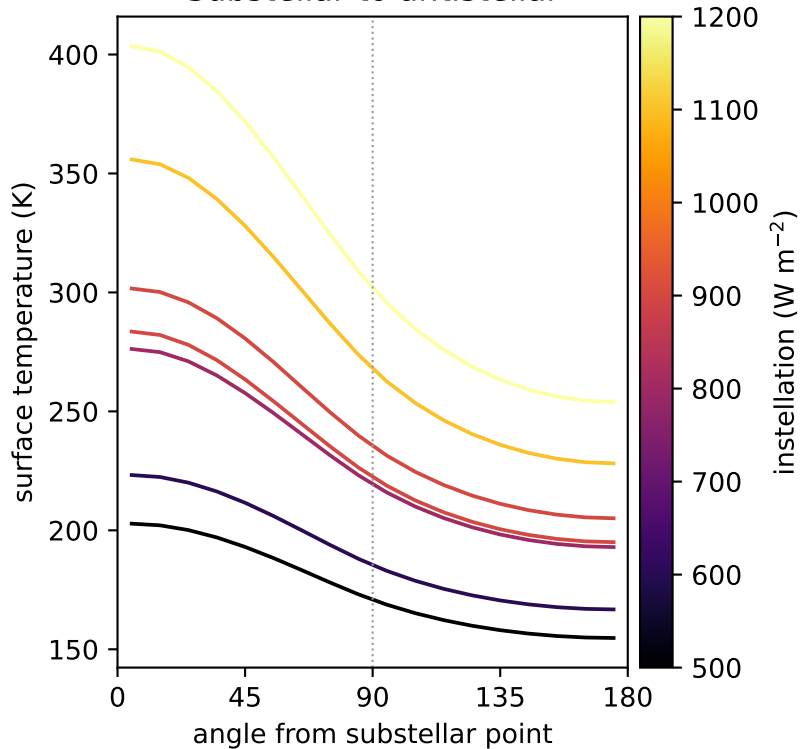
Substellar to antistellar
