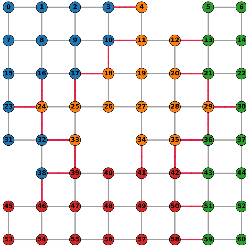
4 patches, partition 4 (23 cut couplers)
