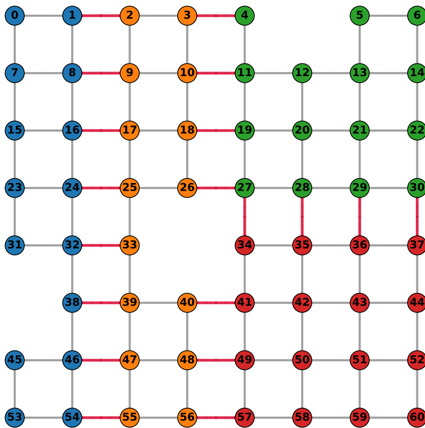
4 patches, partition 1 (22 cut couplers)
