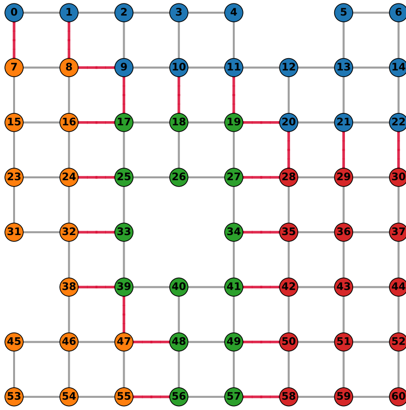
4 patches, partition 2 (22 cut couplers)
