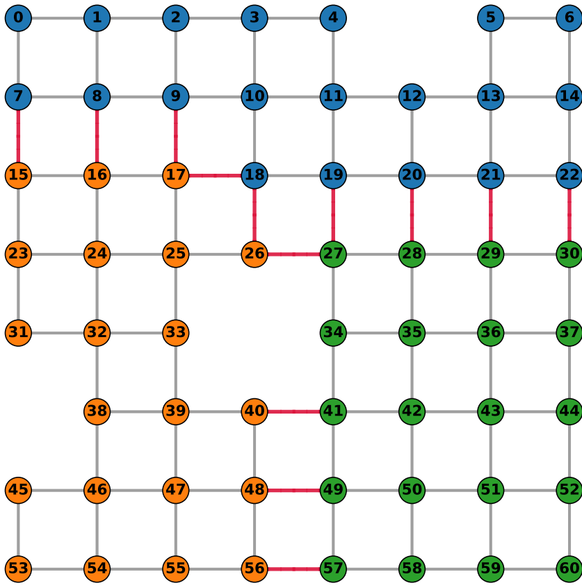
3 patches, partition 2 (13 cut couplers)
