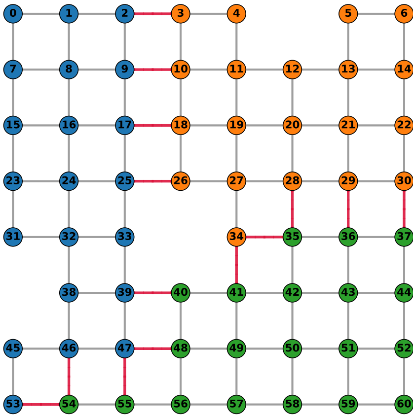
3 patches, partition 4 (14 cut couplers)
