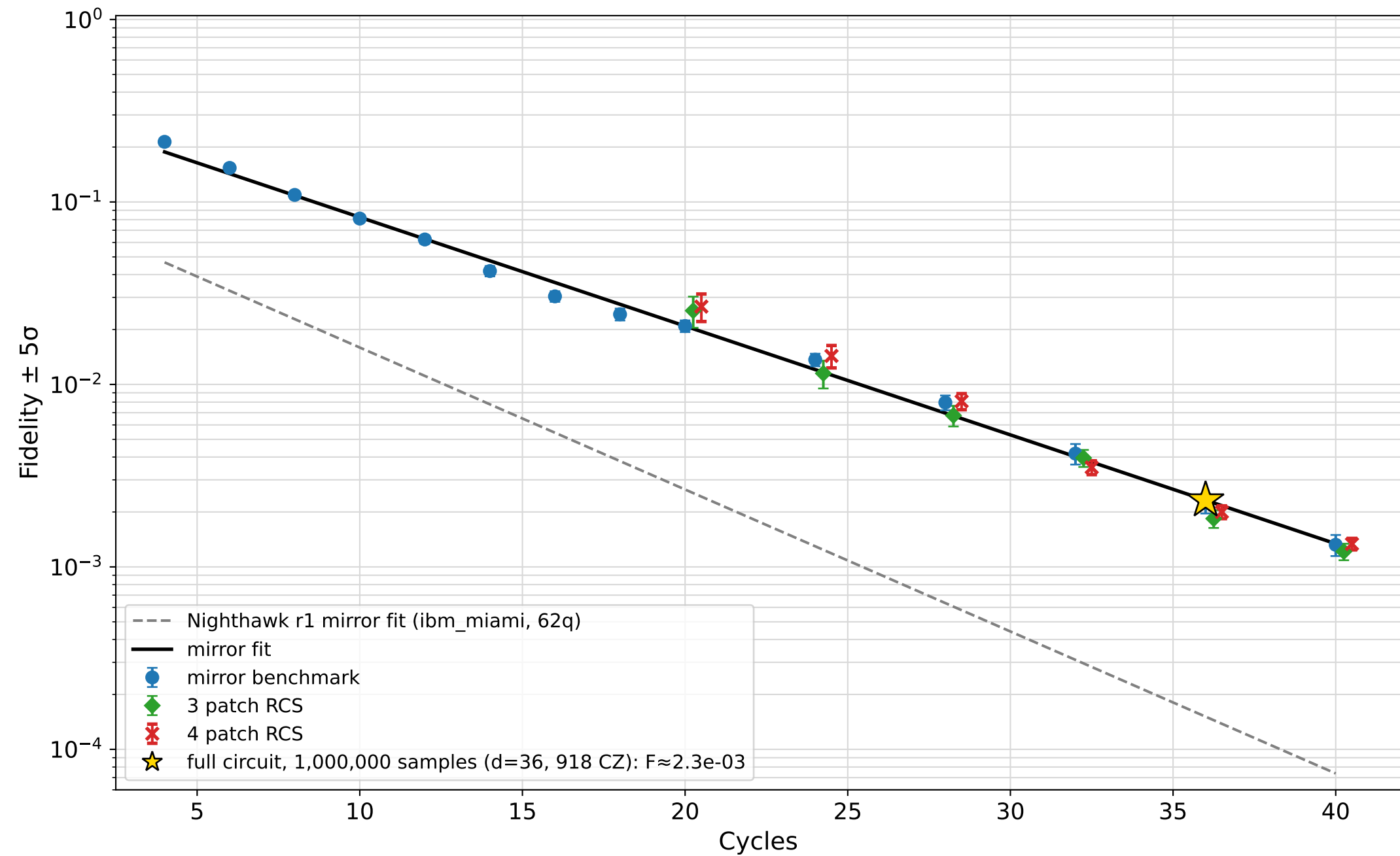
RCS on ibm_phoenix (Nighthawk r2), 61 qubits
