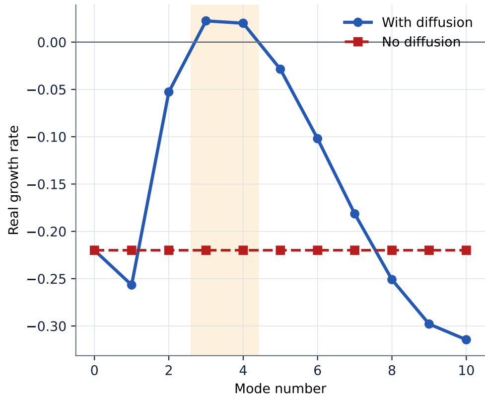
Mode-wise growth at \gamma = 0.0625
