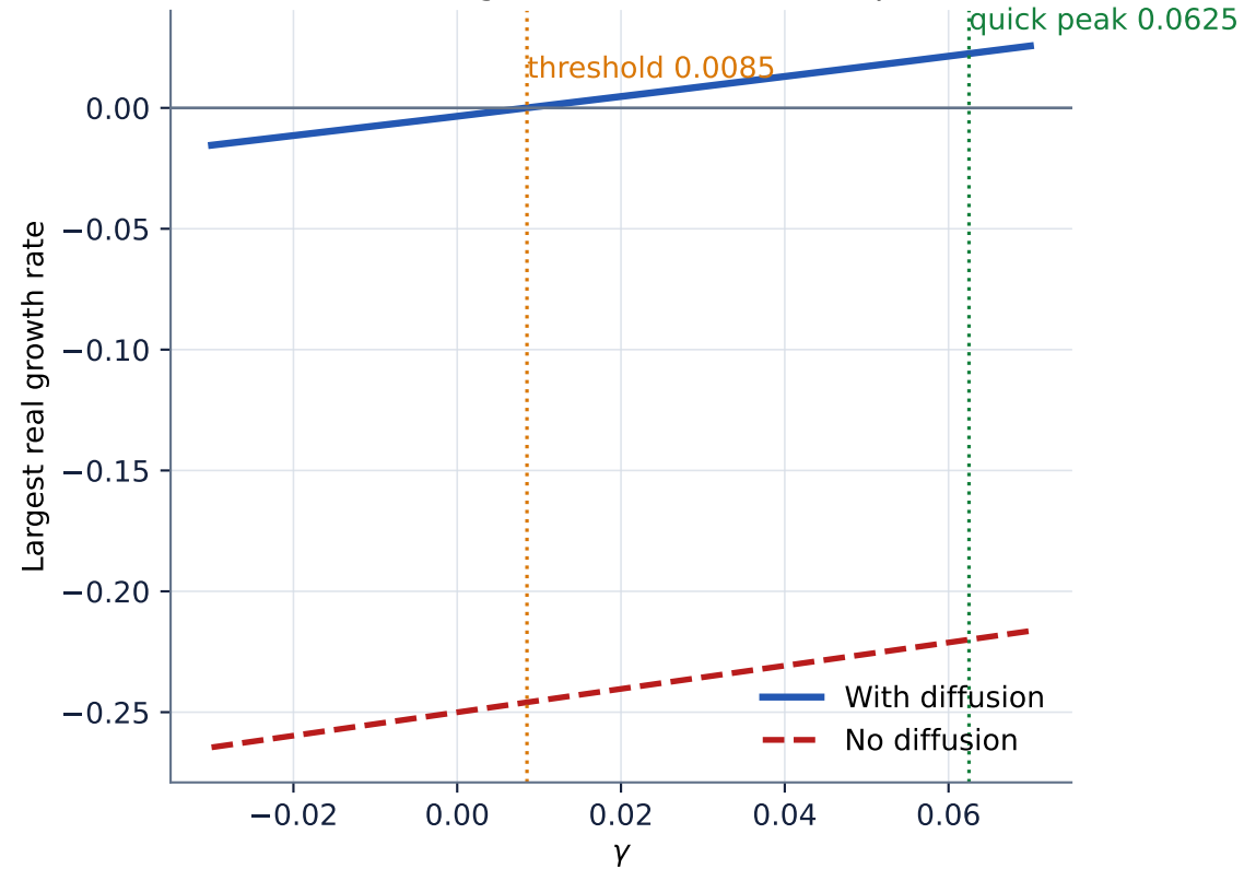
Maximum linear growth rate vs control parameter
