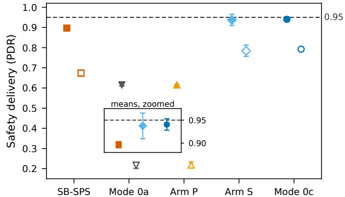
(b) N = 10 ( \lambda_0 = 1 , the critical load)
