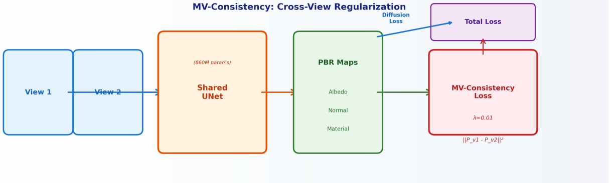
Figure 2: MV-Consistency method overview. Input views are processed through a shared UNet to produce PBR predictions. We add an MSE loss between predictions of different views (red path), which stabilizes training by enforcing cross-view consistency.
