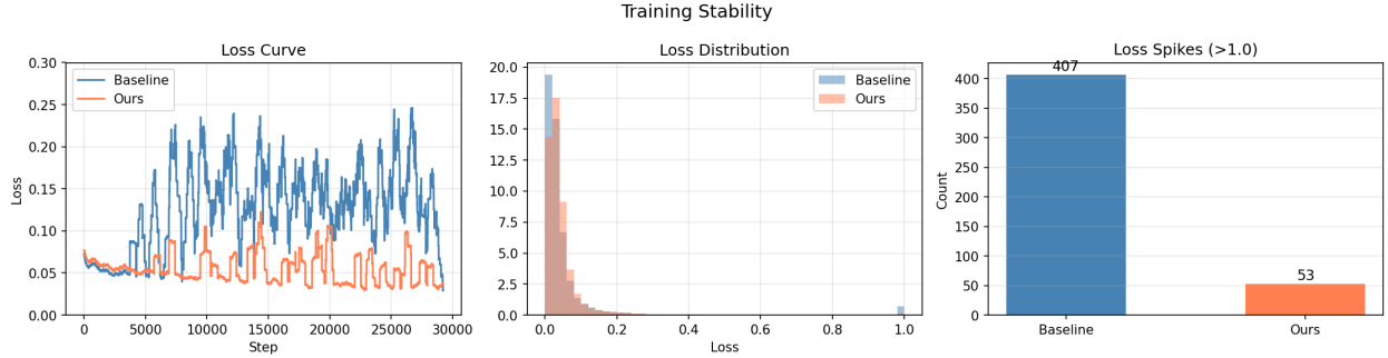
Figure 1: Training stability comparison: (Left) Loss curves showing Baseline spikes vs Ours smooth convergence. (Center) Loss distribution showing Baseline’s heavy tail vs Ours’ compact distribution. (Right) Spike count comparison: 407 vs 53.
