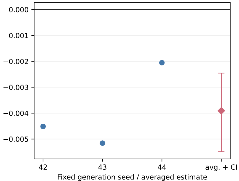
FG-LPIPS
