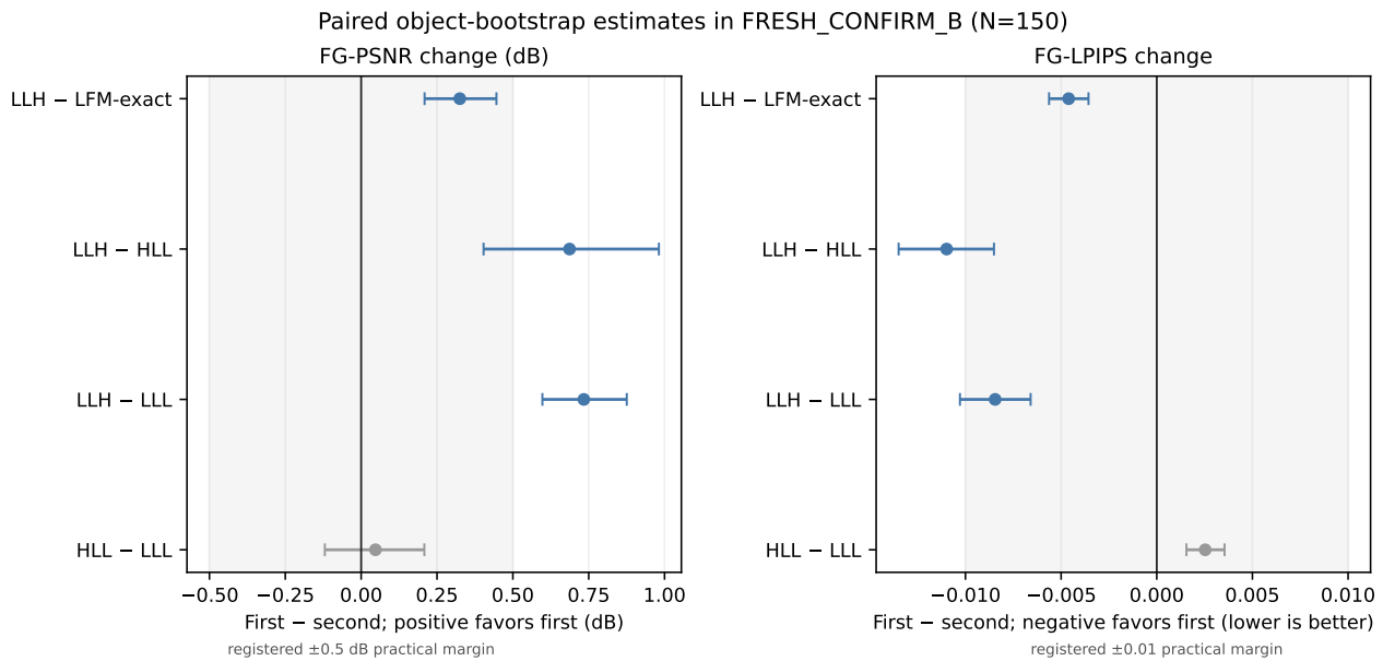
Fig. 2. Paired estimates for the registered LLH contrasts and the separately marked exploratory HLL–LLL contrast. Shaded bands show the predeclared practical margins for LLH–LFM-exact. Confidence intervals describe object resampling; they do not adjust for other endpoints unless the table reports the corresponding Holm family.
