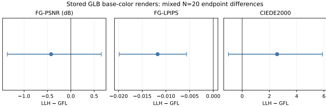
Fig. 4. Stored GLB base-color endpoint differences for LLH minus native GFL. Negative LPIPS and CIEDE2000 favor LLH; positive PSNR favors LLH. The mixed estimates do not establish overall 3D superiority.
