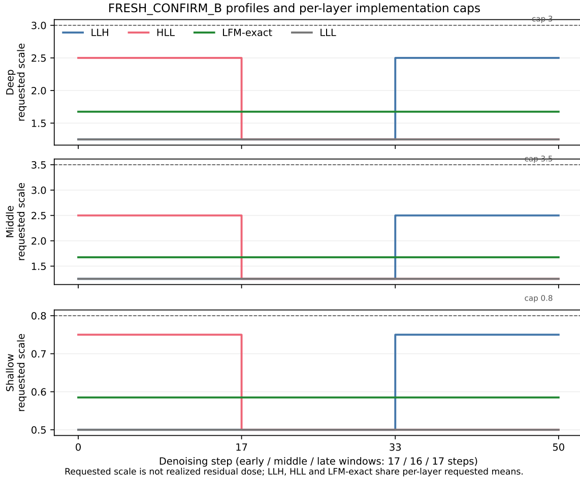
Fig. 1. Requested per-layer scale profiles for the FRESH_CONFIRM_B comparisons. Each temporal window contains 17/16/17 steps. The dashed limits are implementation caps. LLH, HLL, and LFM-exact have the same requested per-layer means; their realized correction norms differ. LLL is the all-low reference.
