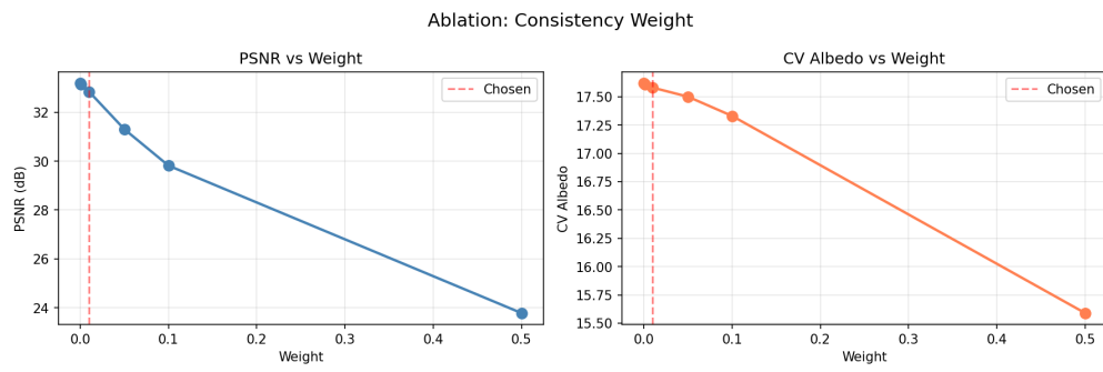
Figure 3: Ablation study: PSNR and Cross-View Consistency vs consistency weight. The red dashed line indicates the chosen weight (0.01).
