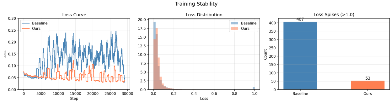
Figure 1: Training stability comparison. Left: Loss curves showing Baseline spikes vs Ours smooth convergence. Center: Loss distribution showing Baseline’s heavy tail vs Ours’ compact distribution. Right: Spike count comparison (407 vs 53).
