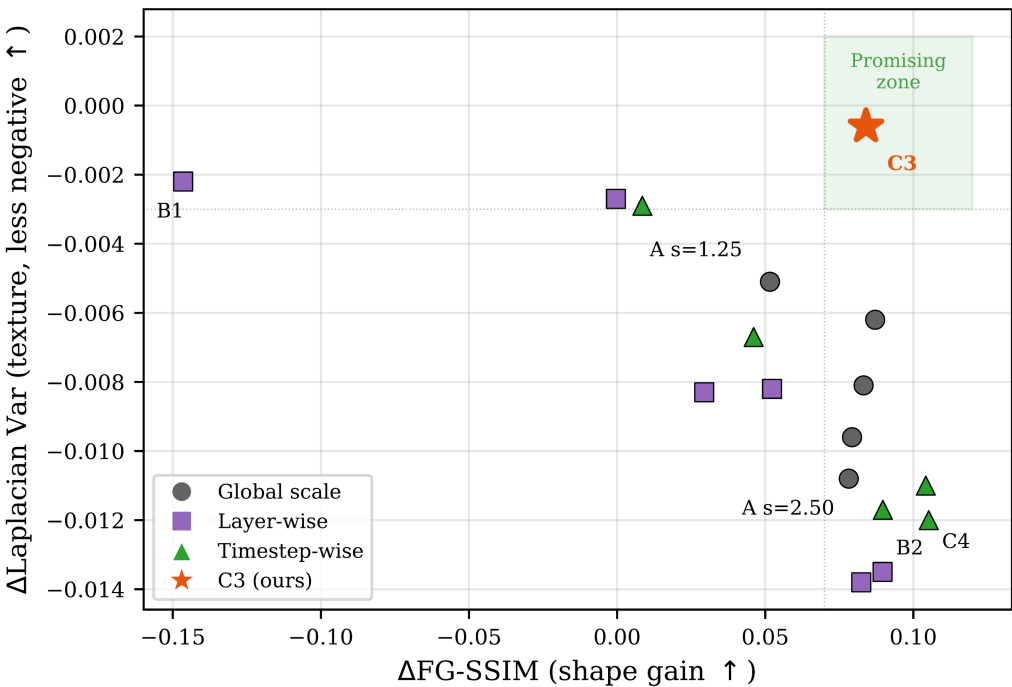
Shape-Texture Trade-off: 17 Scheduling Variants
