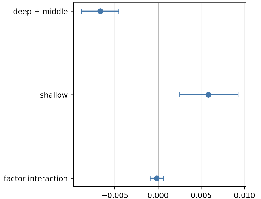
FG-LPIPS
