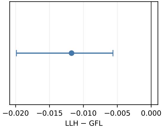
FG-LPIPS
