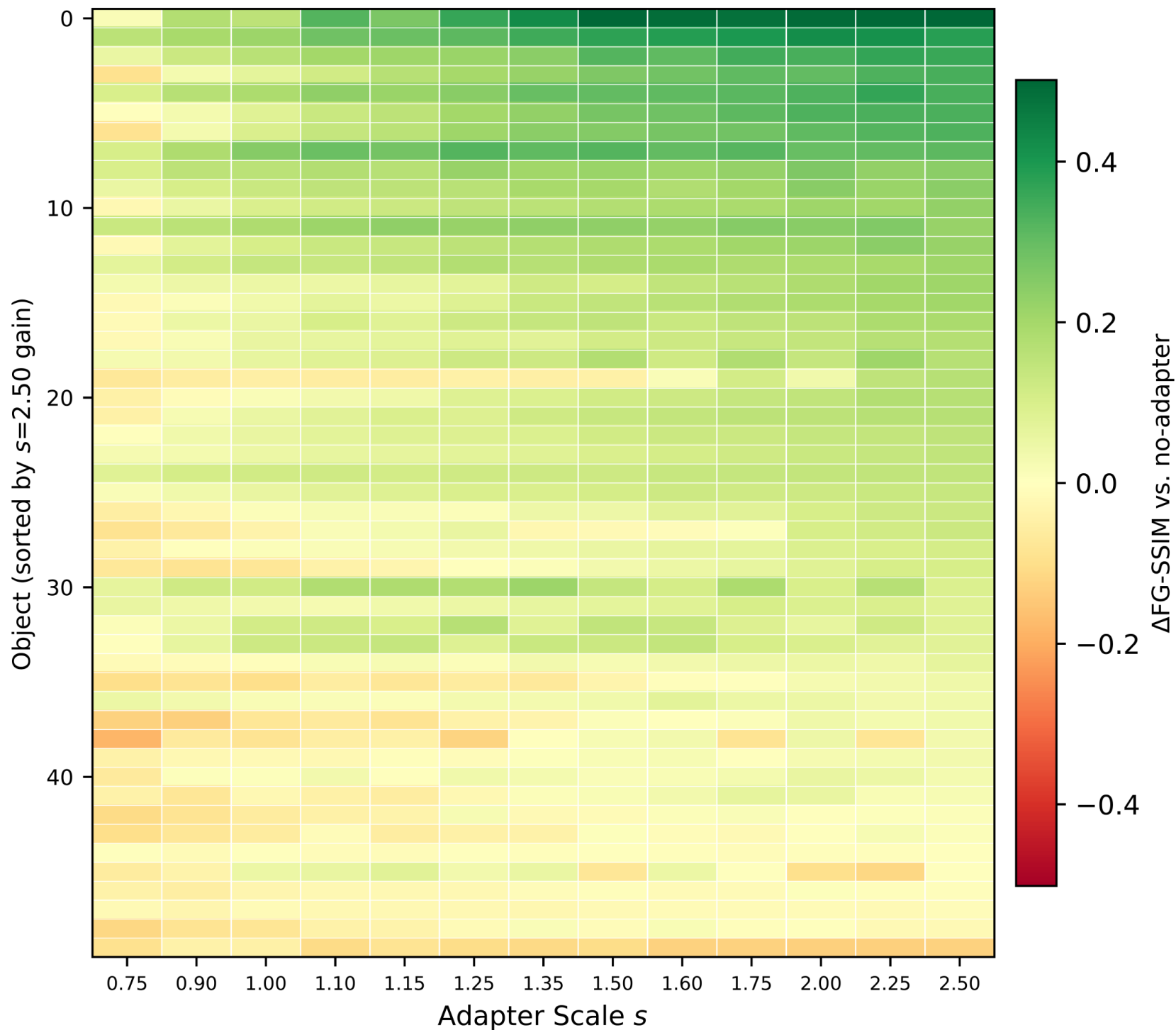
Per-object FG-SSIM improvement across 13 scales (50 objects)
