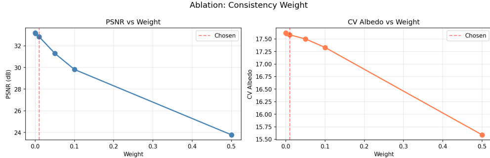
Figure 5: Ablation study: PSNR and Cross-View Consistency vs consistency weight. The red dashed line indicates the chosen weight (0.01).
