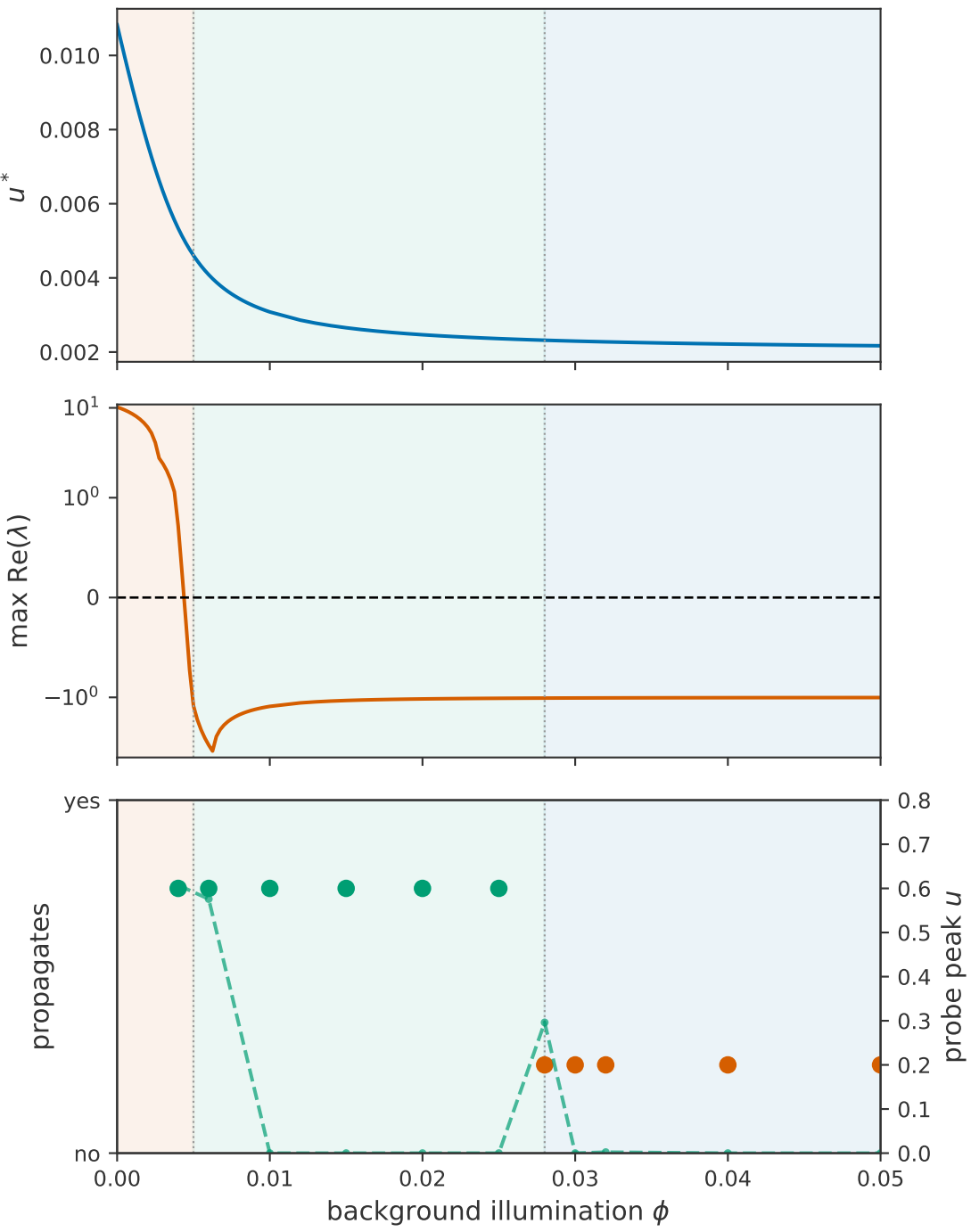
Light-held Oregonator parameter map ( f = 1.4375 , \varepsilon = 0.0501 )
