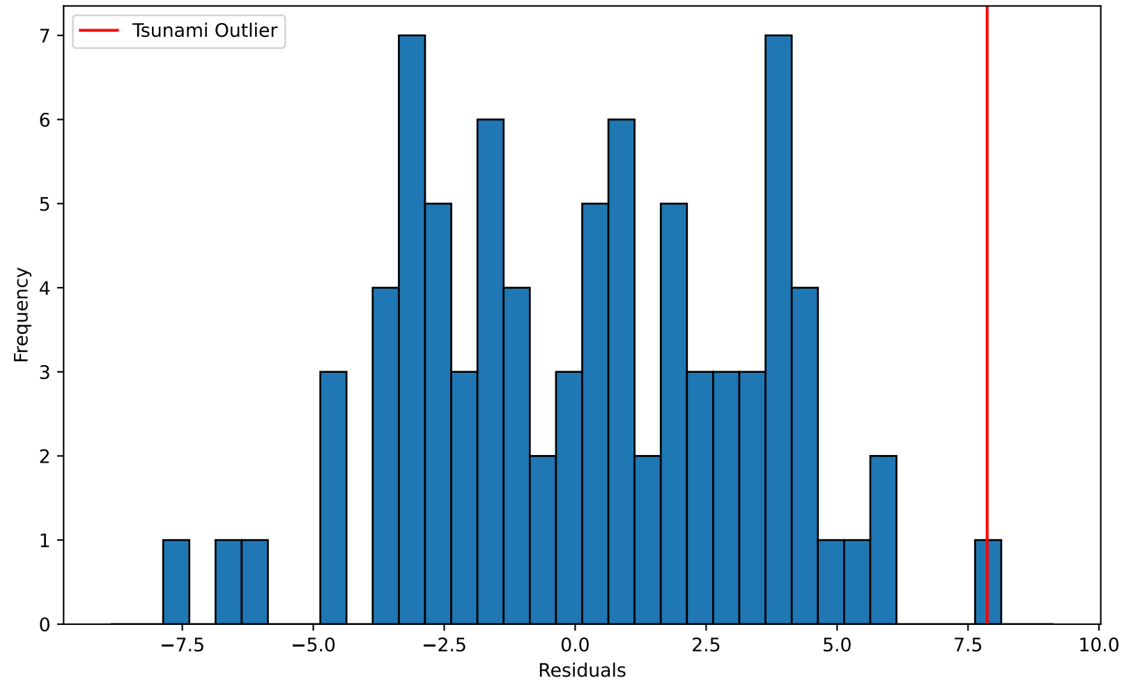
Histogram of Residuals (with Tsunami Outlier)
