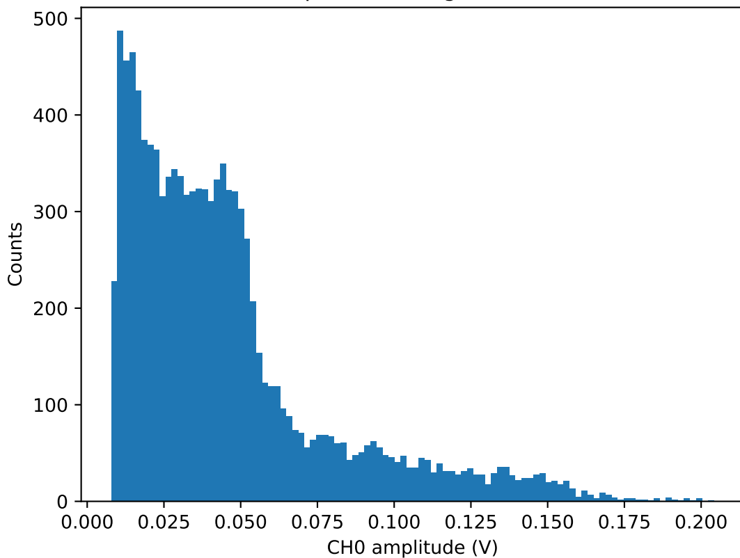
CH0 Amplitude histogram for 44.0V
