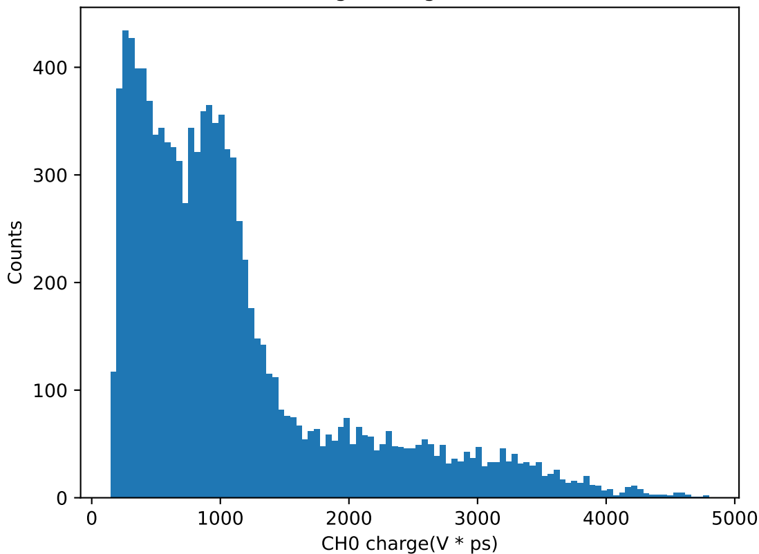
CH0 Charge histogram for 42.5V
