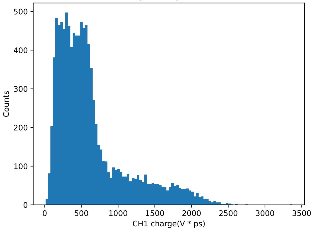
CH1 Charge histogram for 42.0V
