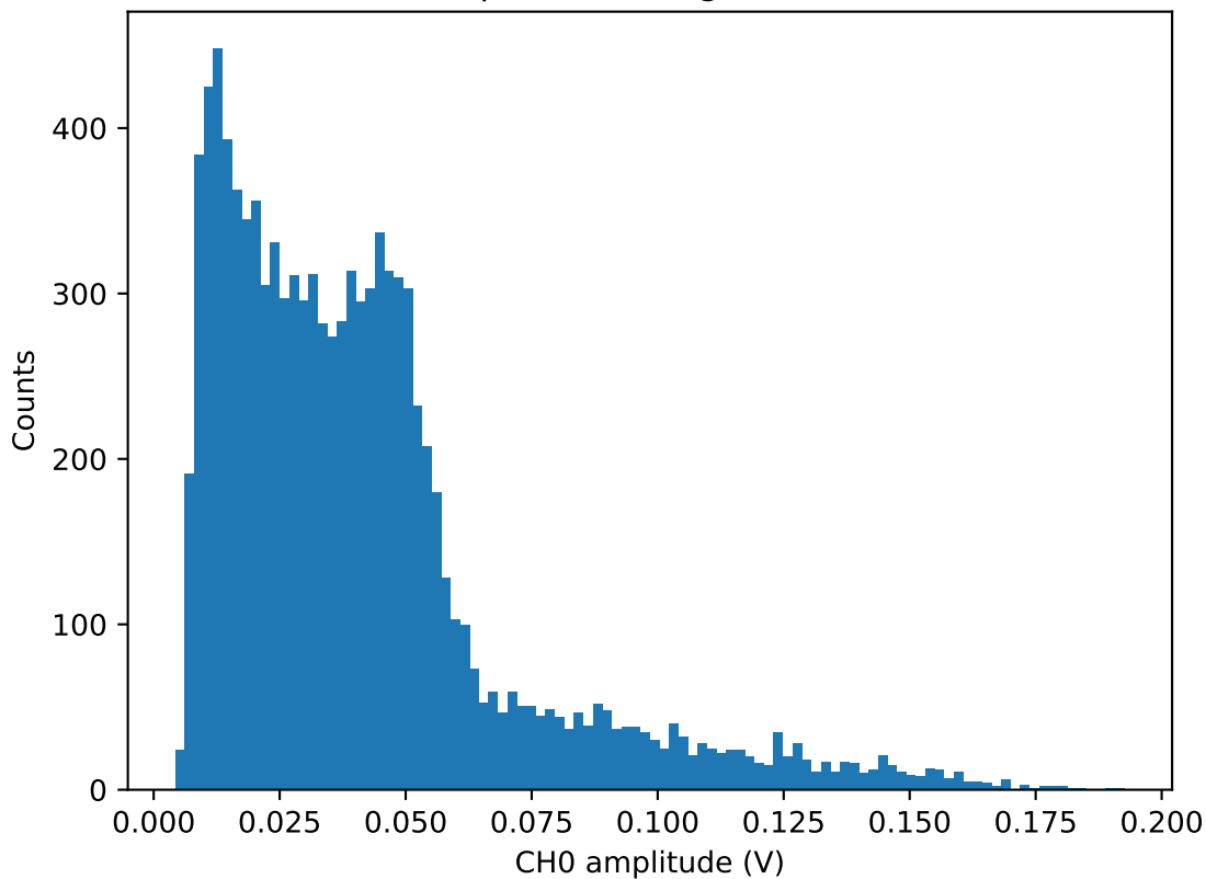
CH0 Amplitude histogram for 45.0V
