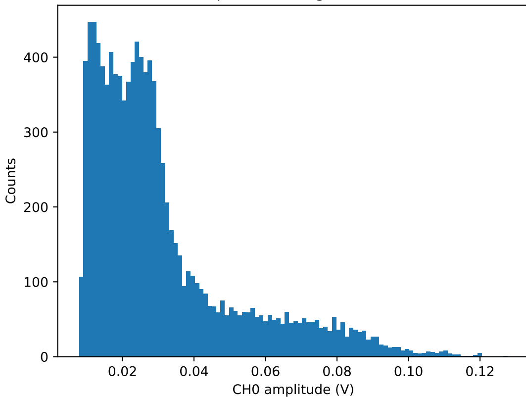
CH0 Amplitude histogram for 42.0V
