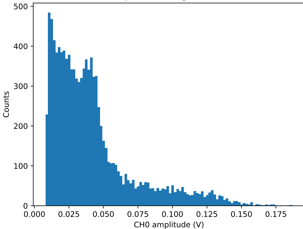
CH0 Amplitude histogram for 43.5V
