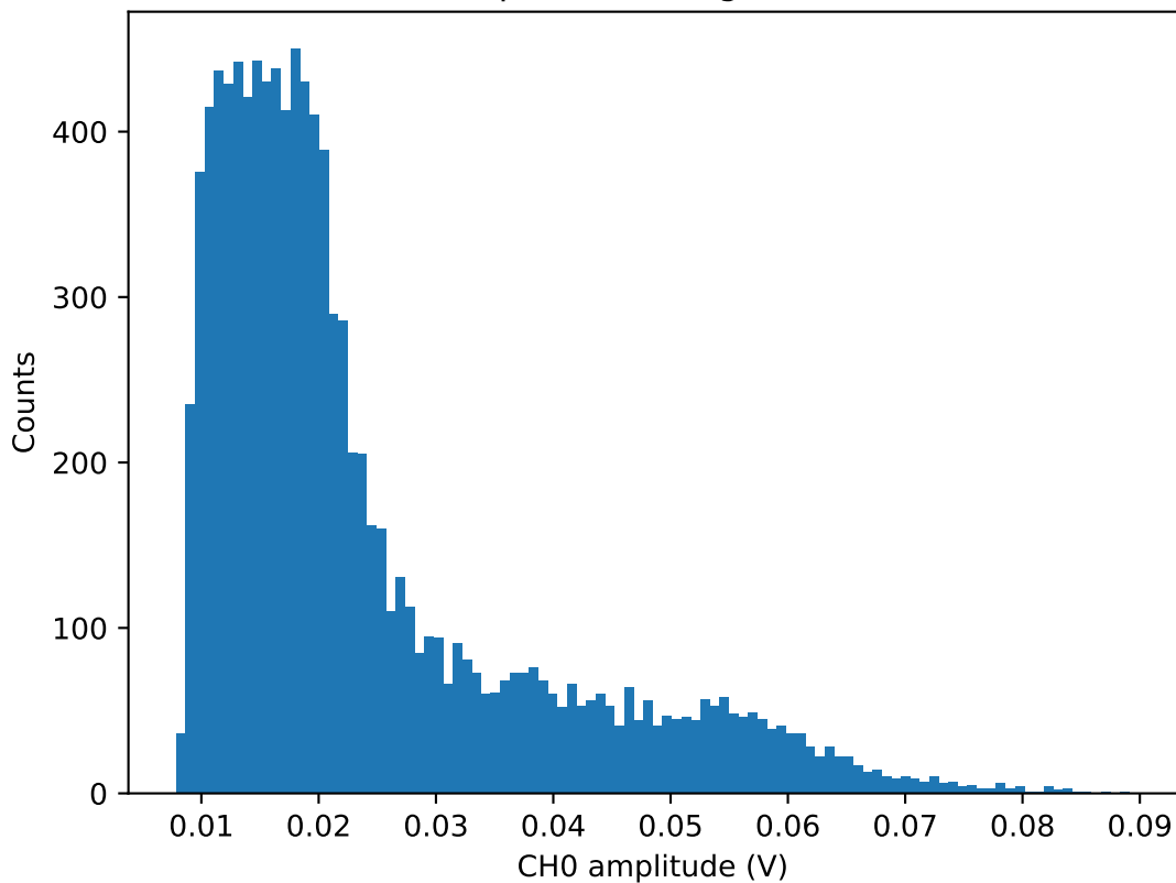
CH0 Amplitude histogram for 41V
