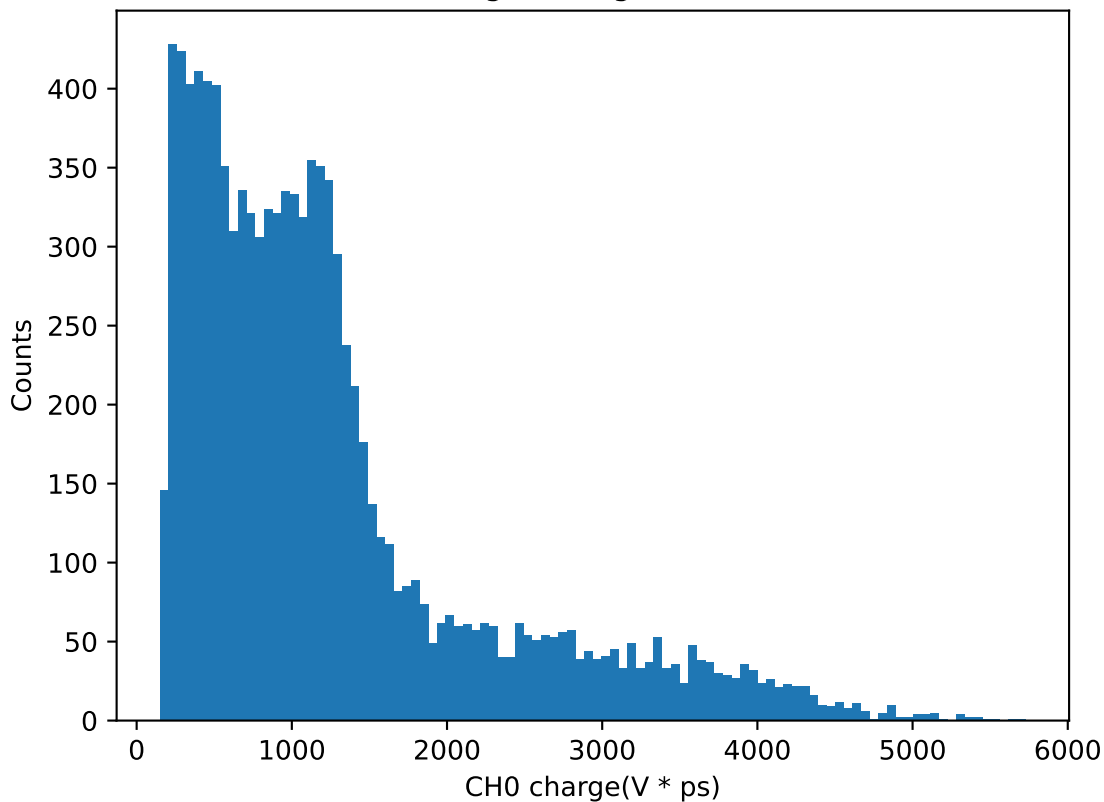
CH0 Charge histogram for 43.0V
