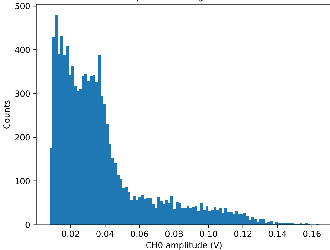
CH0 Amplitude histogram for 43.0V
