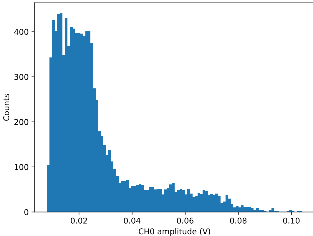
CH0 Amplitude histogram for 41.5V
