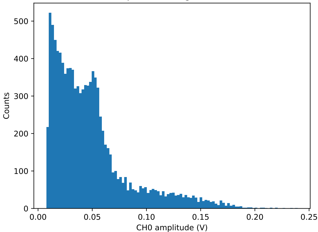
CH0 Amplitude histogram for 44.5V
