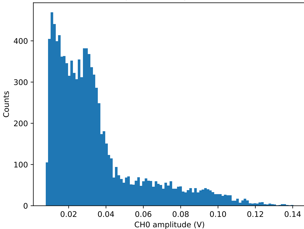
CH0 Amplitude histogram for 42.5V
