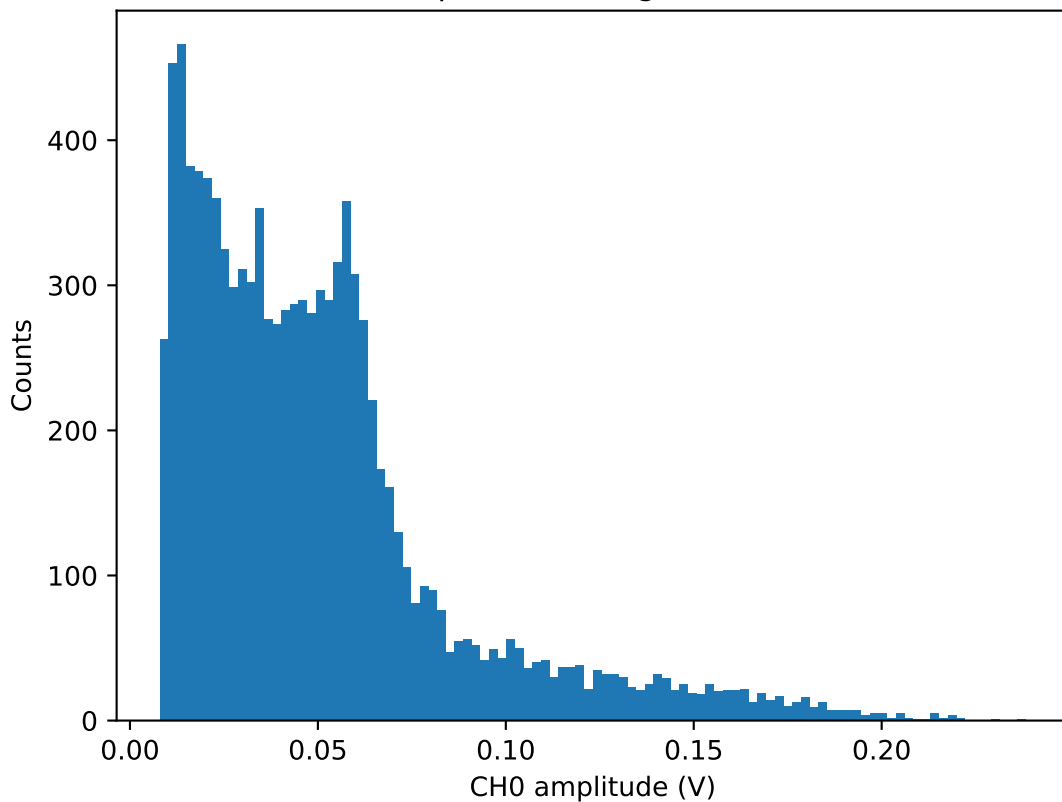
CH0 Amplitude histogram for 45.0V
