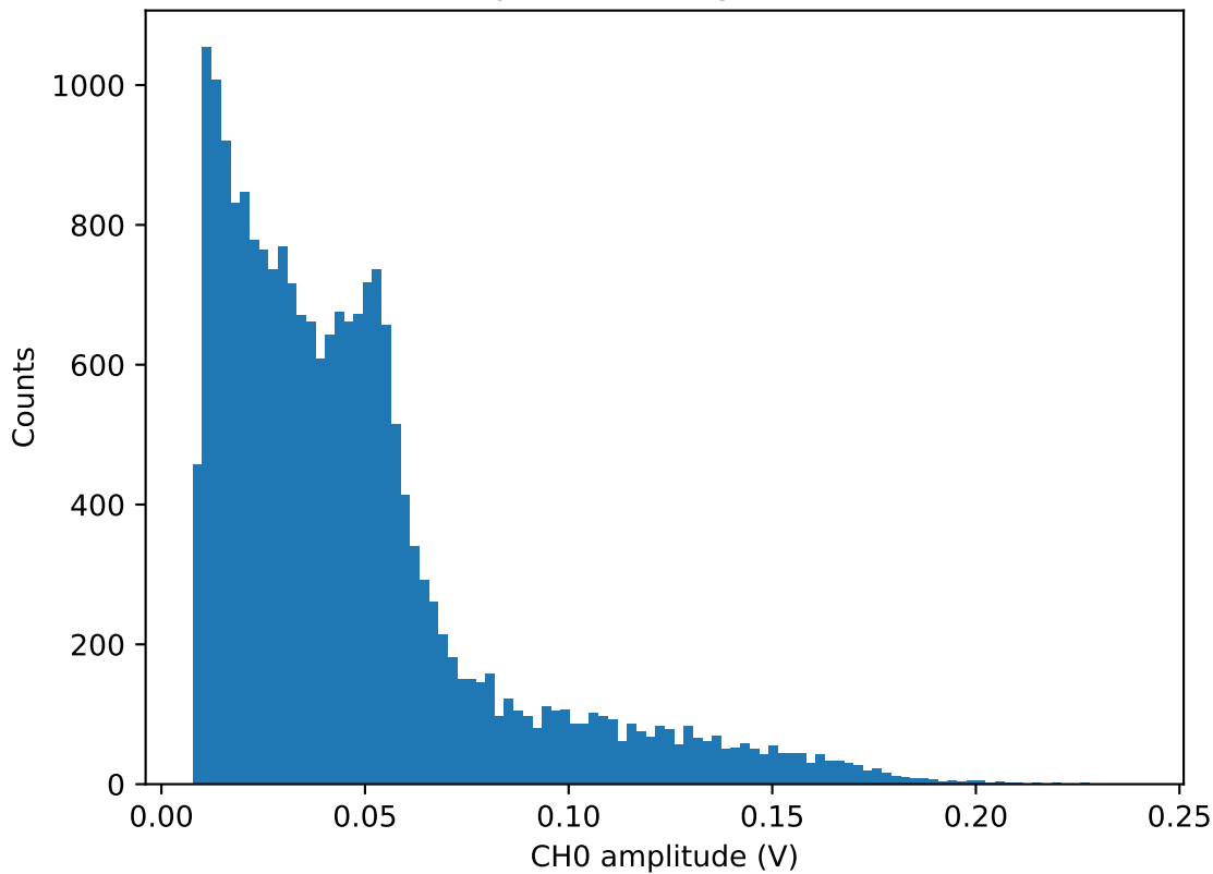
CH0 Amplitude histogram for 44.5V
