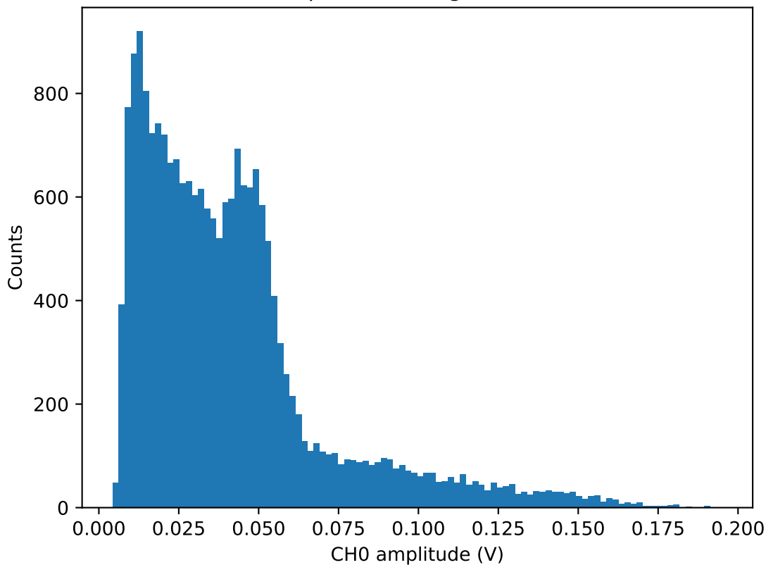
CH0 Amplitude histogram for 45.0V
