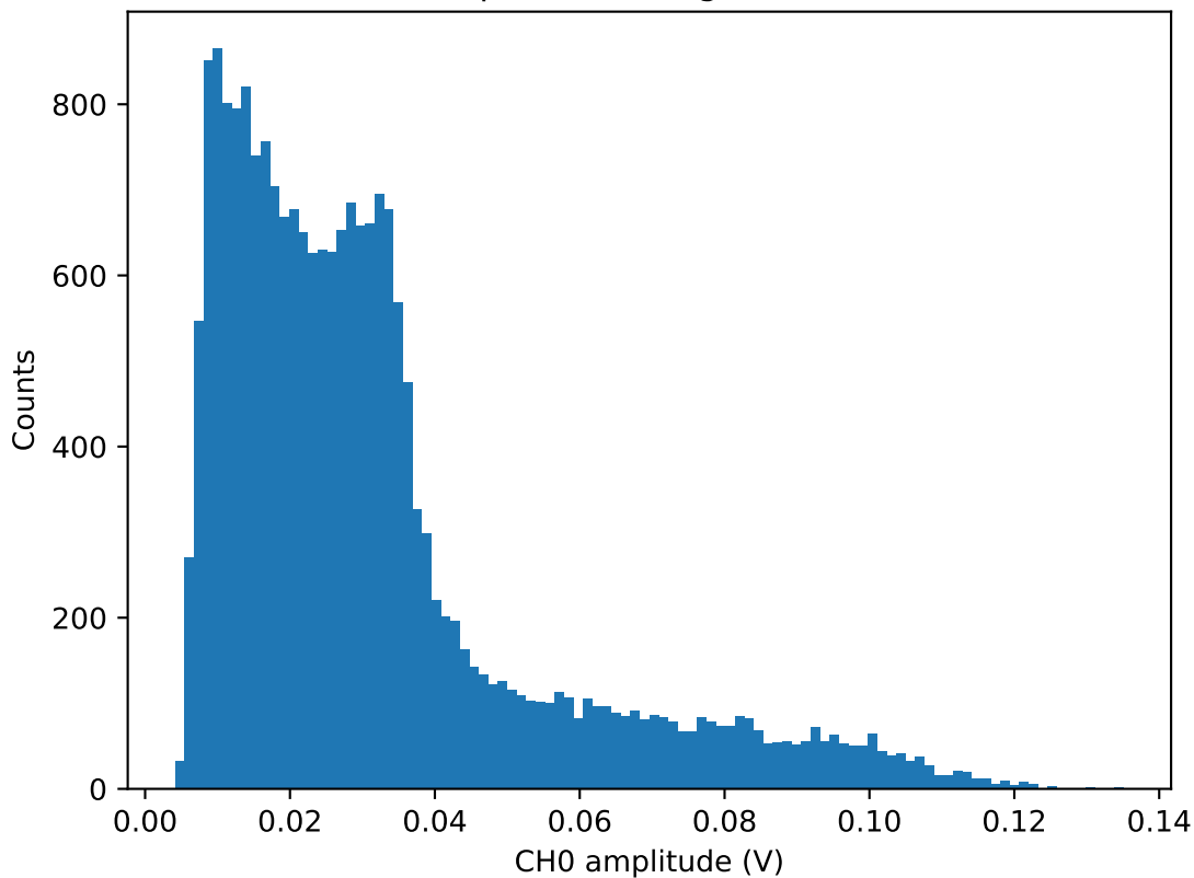
CH0 Amplitude histogram for 43.5V
