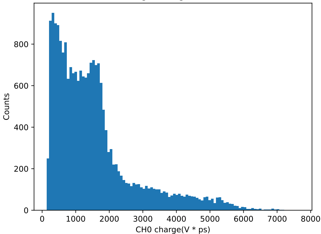
CH0 Charge histogram for 44.0V
