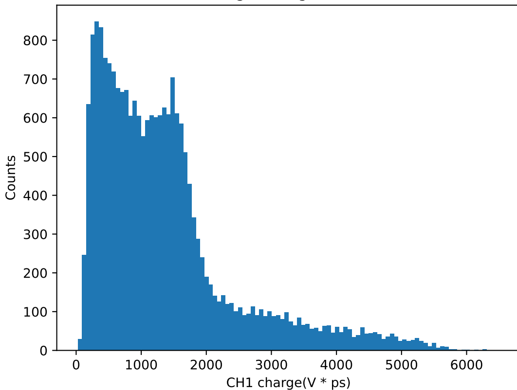
CH1 Charge histogram for 44.5V
