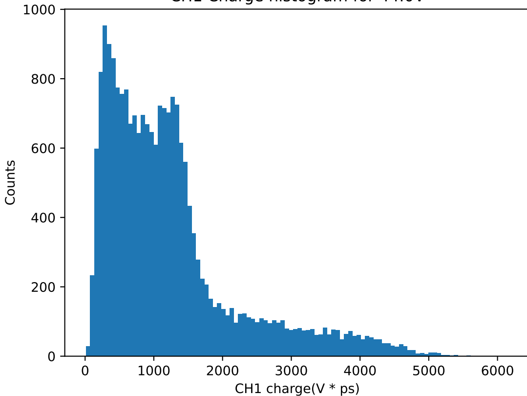
CH1 Charge histogram for 44.0V
