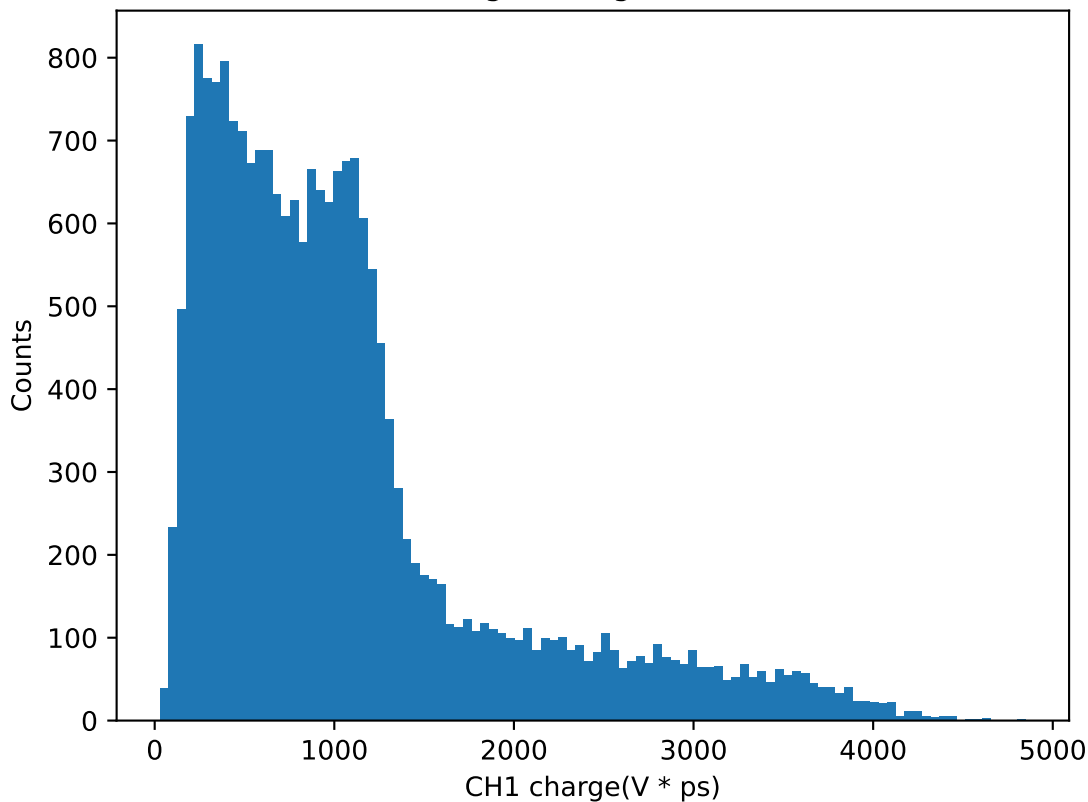
CH1 Charge histogram for 43.5V
