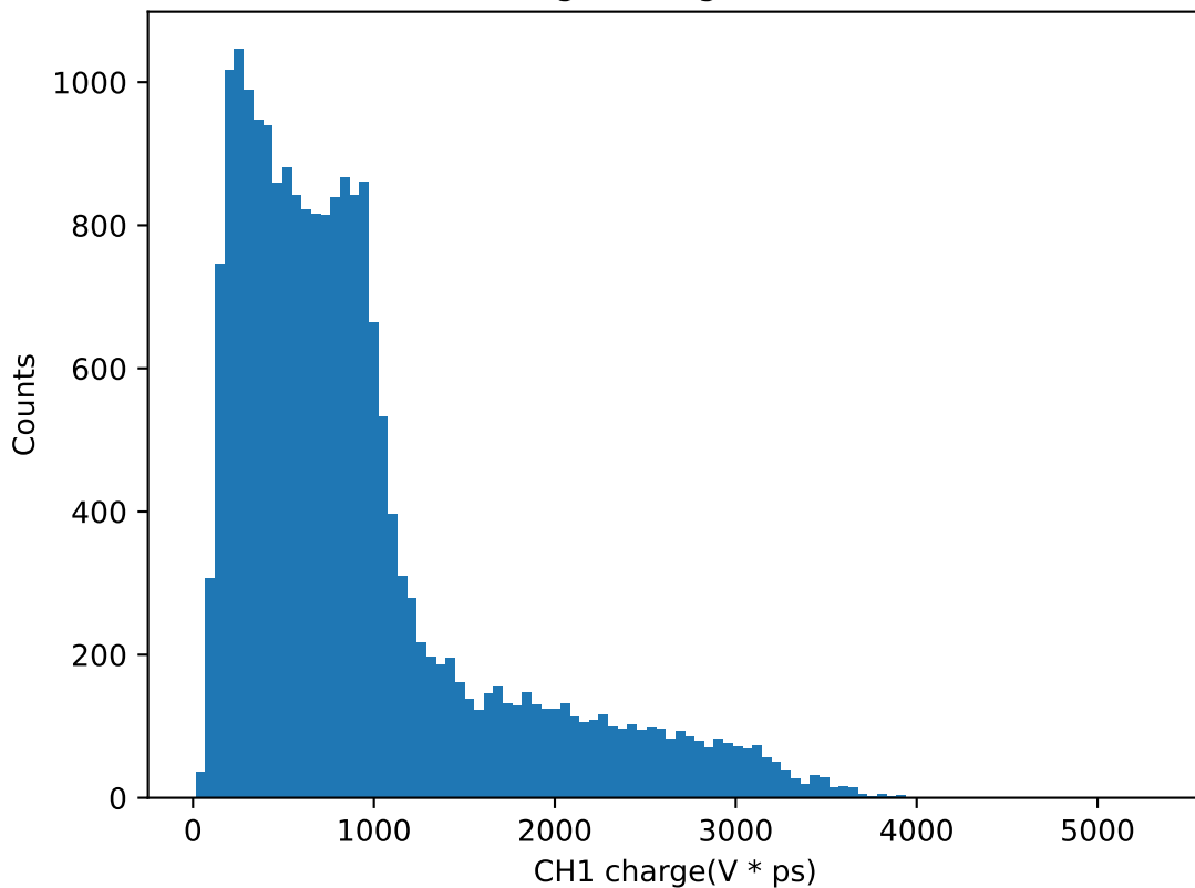
CH1 Charge histogram for 43.0V
