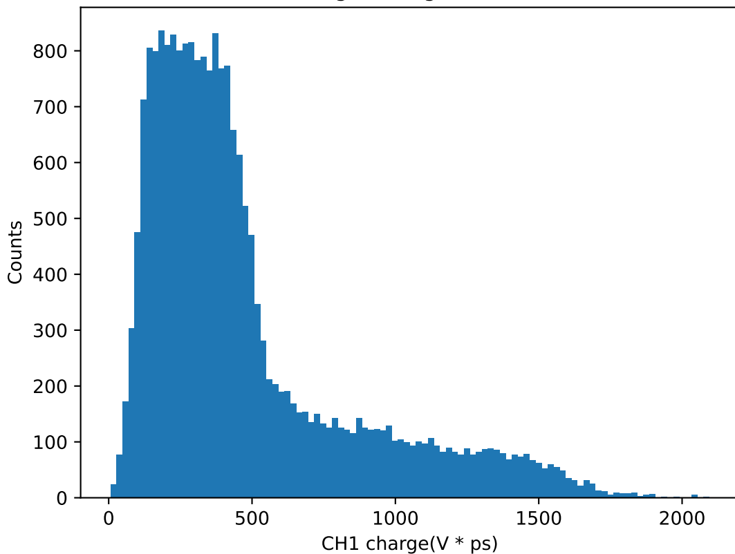
CH1 Charge histogram for 41.5V
