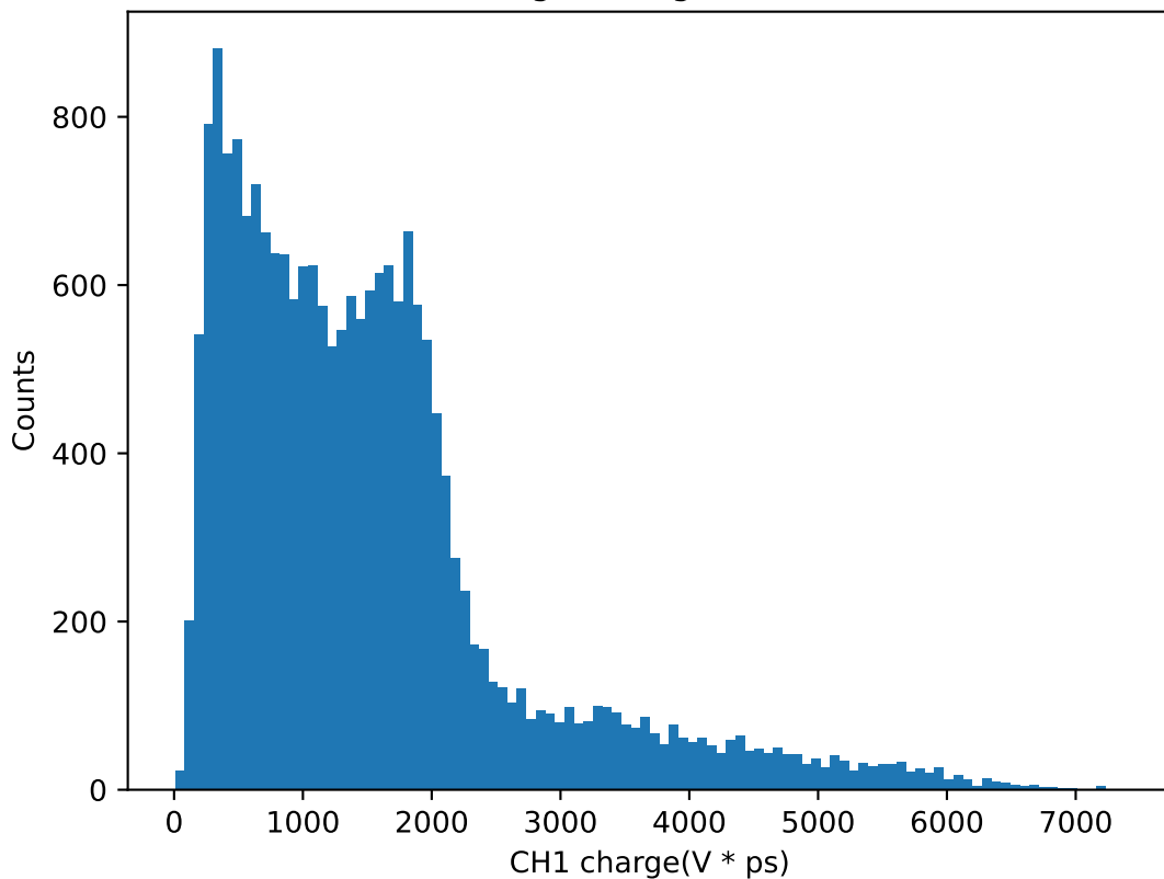
CH1 Charge histogram for 45.0V
