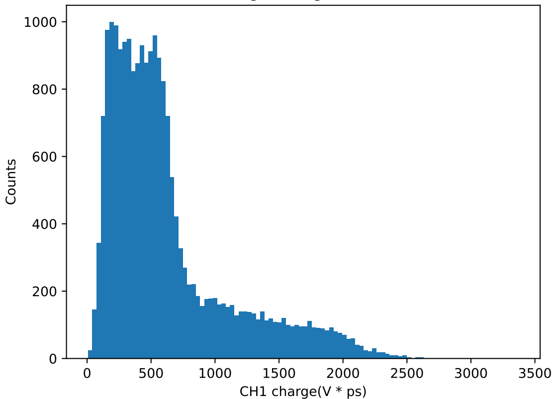
CH1 Charge histogram for 42.0V
