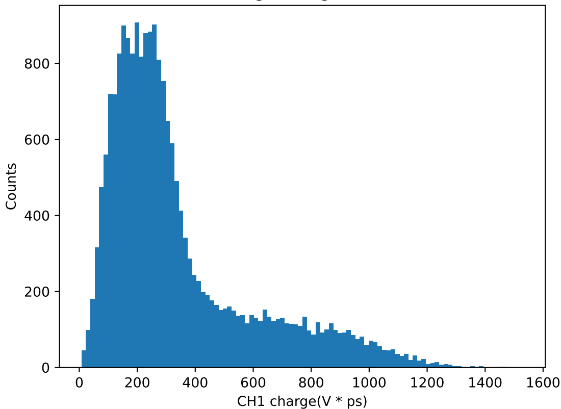
CH1 Charge histogram for 41V
