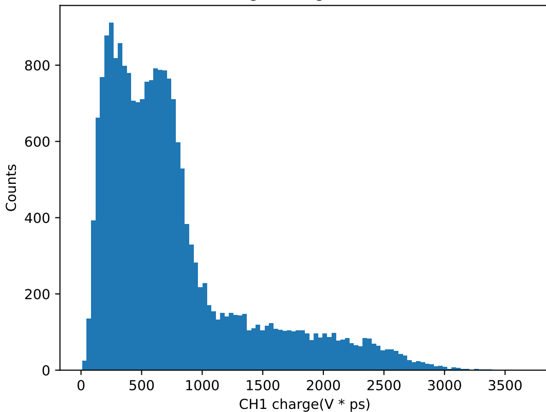
CH1 Charge histogram for 42.5V
