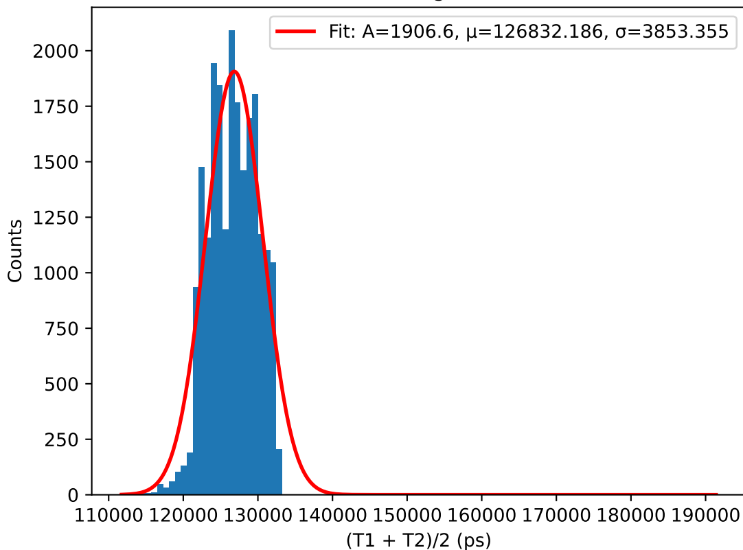
(T1 + T2)/2 histogram for 42.0V
