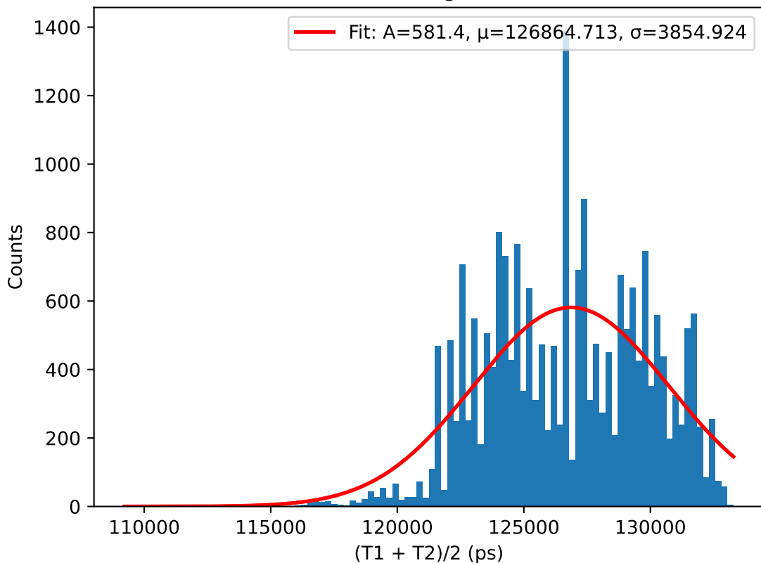
(T1 + T2)/2 histogram for 42.5V
