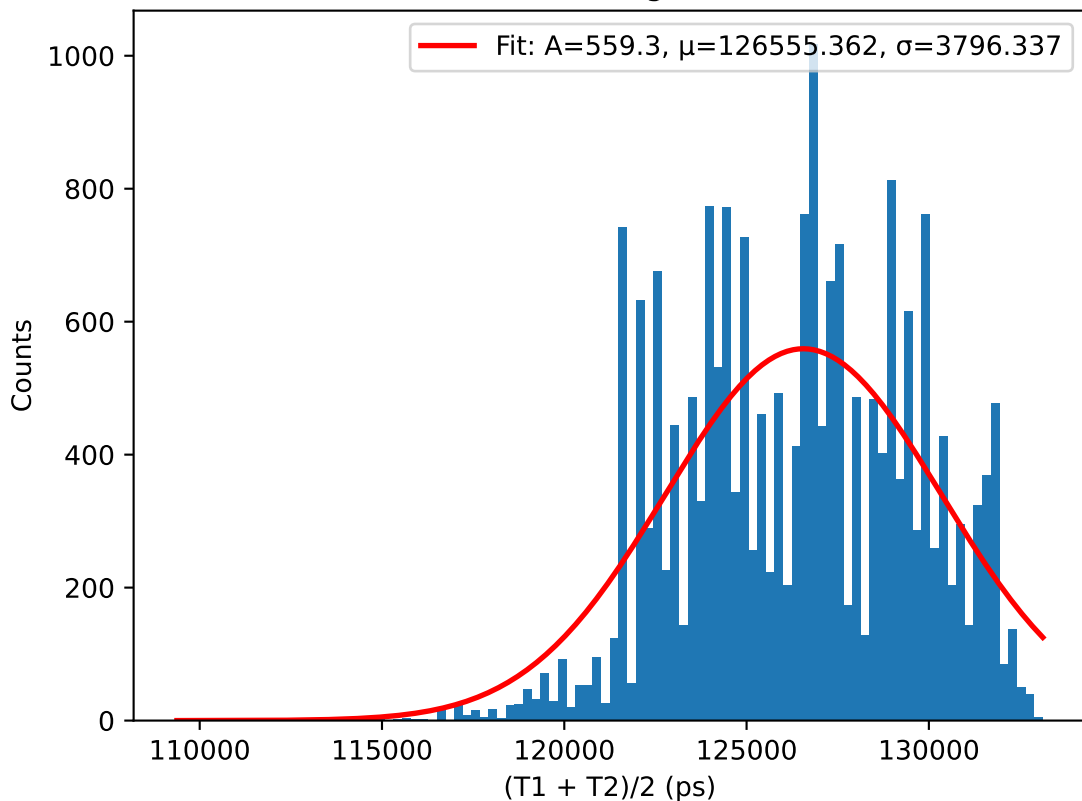
(T1 + T2)/2 histogram for 41V
