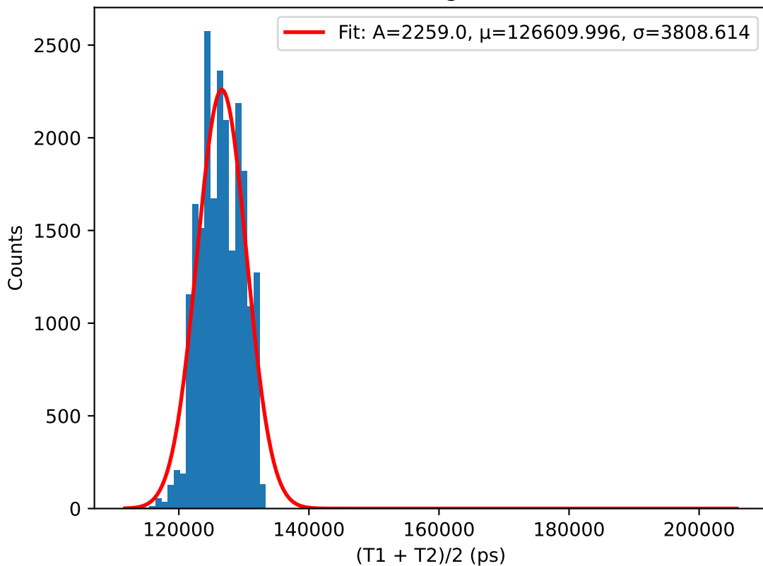
(T1 + T2)/2 histogram for 41.5V
