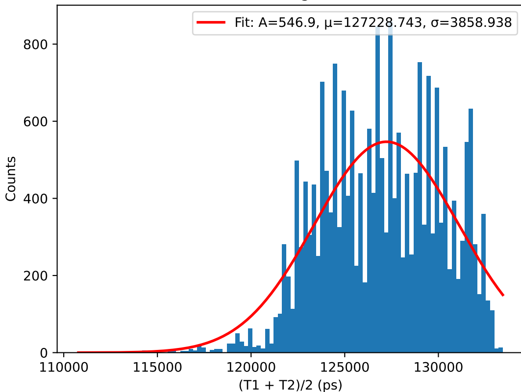
(T1 + T2)/2 histogram for 44.0V
