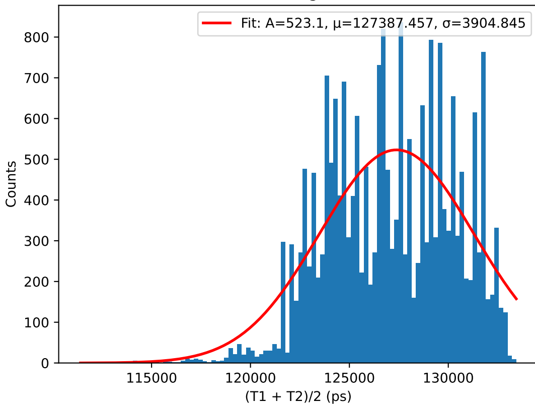
(T1 + T2)/2 histogram for 44.5V
