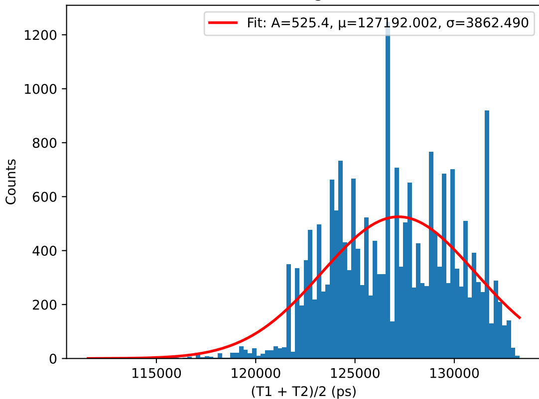
(T1 + T2)/2 histogram for 43.5V
