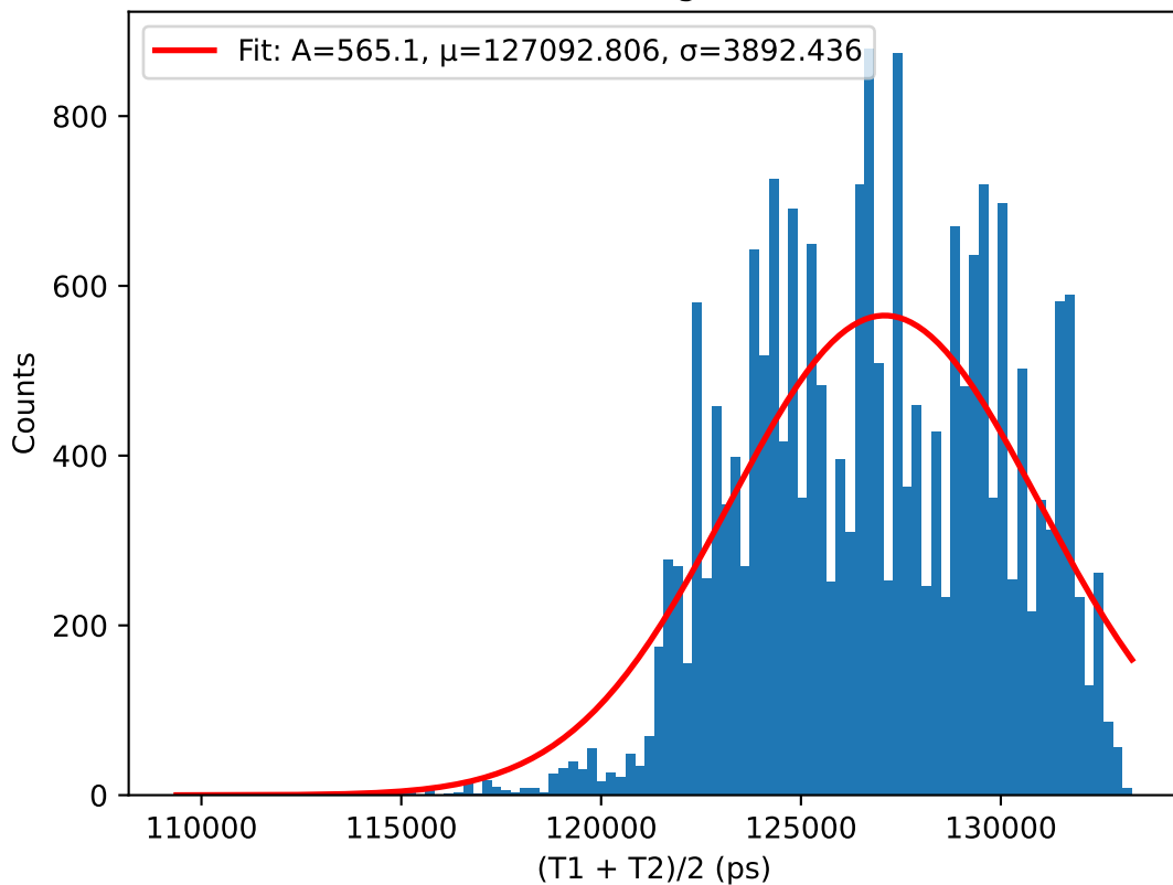
(T1 + T2)/2 histogram for 43.0V
