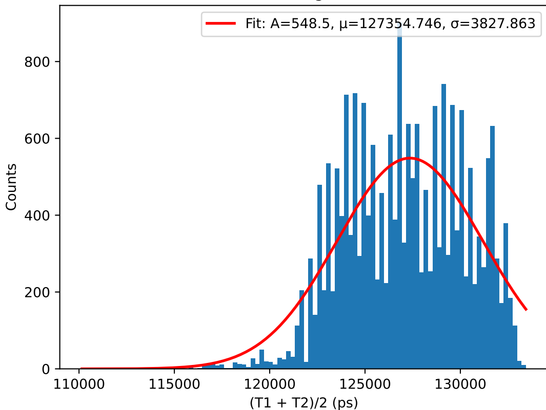
(T1 + T2)/2 histogram for 45.0V
